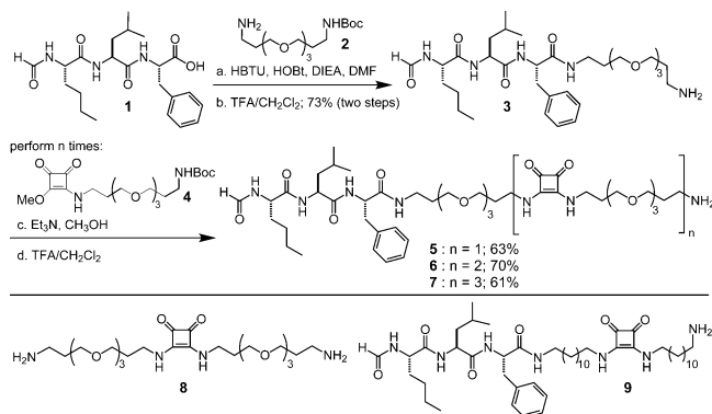
Scheme 1. Route to Formyl Peptides Designed To Bind to FPR
