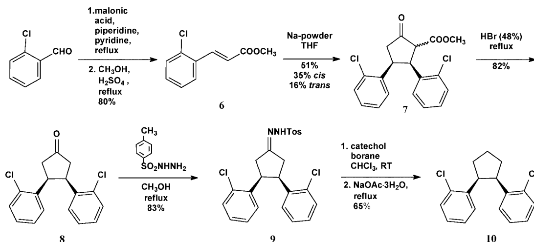
Scheme 7. Synthesis of 15
