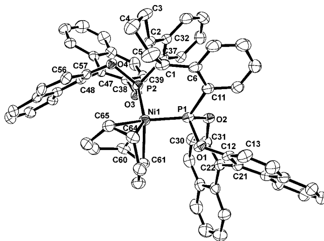
Figure 5. ORTEP representation of (2-\kappa^2P)Ni(COD) . Thermal ellipsoids are drawn at 50% probability; hydrogen atoms are omitted for clarity. Selected interatomic distances (Å) and angles (deg): Ni1–P1 = 2.1214(10), Ni1–P2 = 2.1052(10), Ni1–C60 = 2.147(4), Ni1–C61 = 2.177(4), Ni1–C64 = 2.119(4), Ni1–C65 = 2.116(4), P2–Ni1–P1 = 101.67(4) , P1–Ni1–C60 = 128.18(11) , P2–Ni1–C61 = 128.82(11) , P1–Ni1–C61 = 97.83(11) .
