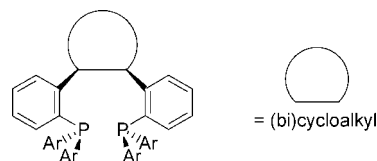
Scheme 3. A New Class of Chelating Trisaryl Bisphosphorus Ligands for Rhodium-Catalyzed Hydroformylation Reactions
