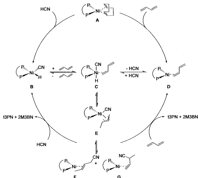
Scheme 2. Proposed Catalytic Cycles for 1,3-Butadiene Hydrocyanation and Isomerization of 2M3BN
