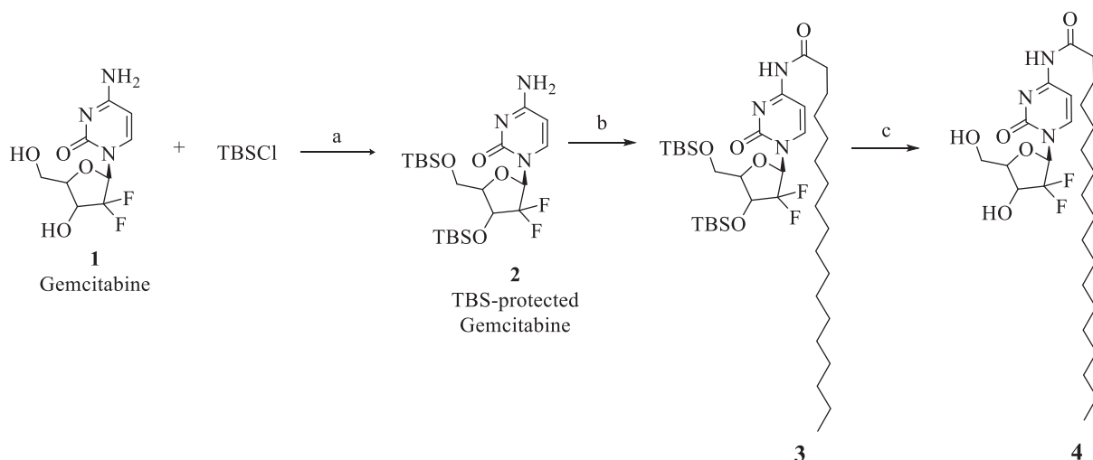
Scheme 1. Reagents and conditions for the synthesis of 4NSG (4): a) TBSCl, imidazole, DCM, rt. b) DIPEA, stearic anhydride, DCM, 24 h c) TBAF DMF, rt., 2 h.
