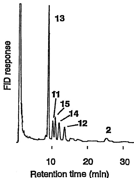
Fig. 1. Product Distribution Pattern of the Leu607Phe Mutant by a GC Analysis.
