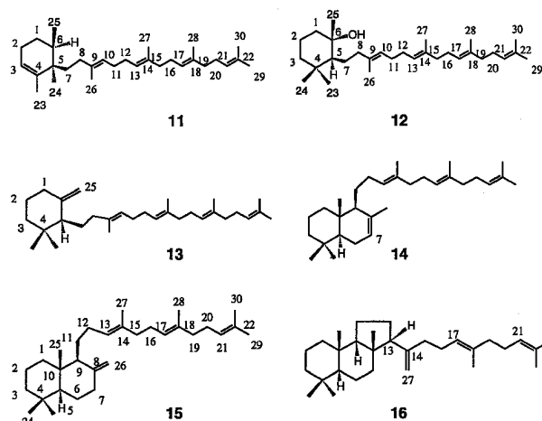
Fig. 2. Structures of the Abortive Cyclization Products Isolated by Some Mutated SHCs Constructed in This Paper.
