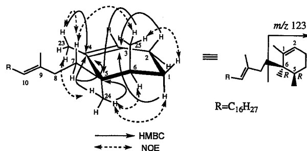
Fig. 3. Selected HMBC, NOEs and EI-MS Fragment Ion ( m/z 123, base peak) Data for the Structural Determination of 11 .
