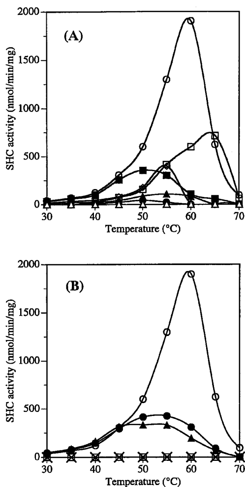
Fig. 4. Specific Enzyme Activities of the Mutated and Wild-type SHCs Plotted against the Incubation Temperatures, These Being Estimated from the Production of Hopene 2 .
