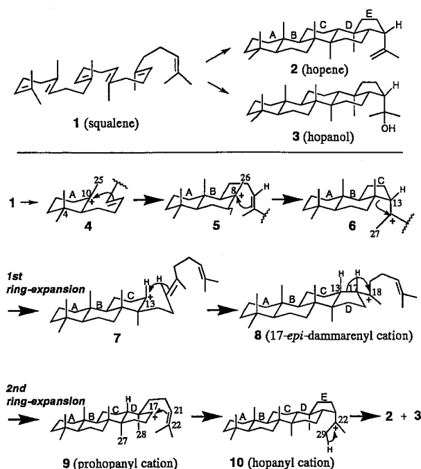
Scheme 1. Polycyclization Reaction of Squalene 1 , Leading to Hopene 2 and Hopanol 3 .
