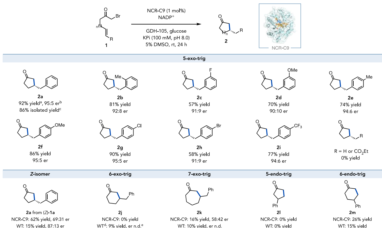
Figure 2. Directed evolution of NCR catalysts for non-natural asymmetric radical cyclization. (A) Chemoselectivity (cyclization versus debrominative hydrogenation), stereoselectivity, and yields improvement of NCR variants over wild-type NCR. Standard reaction conditions: the reaction mixture (500 \mu L) consisted of model substrate ( 1a , 0.004 mmol), GDH-105 (0.5 mg), glucose (5.0 mg), NADP + (0.5 mg), and purified NCR variants (1.0 mol %) in buffer (100 mM KPi buffer pH 8.0) with 5% DMSO as cosolvent at room temperature for 24 h. Yields were determined via HPLC relative to an internal standard (average of triplicate). Enantiomeric ratio (er) was determined via HPLC on a chiral stationary phase. (B) Crystal structure of wild-type NCR (PDB: 4s3u). Residues for substrate binding (H172 and N175) are shown as blue sticks. Four beneficial sites Y343, F269, W342, and I231 are shown in orange sticks.
