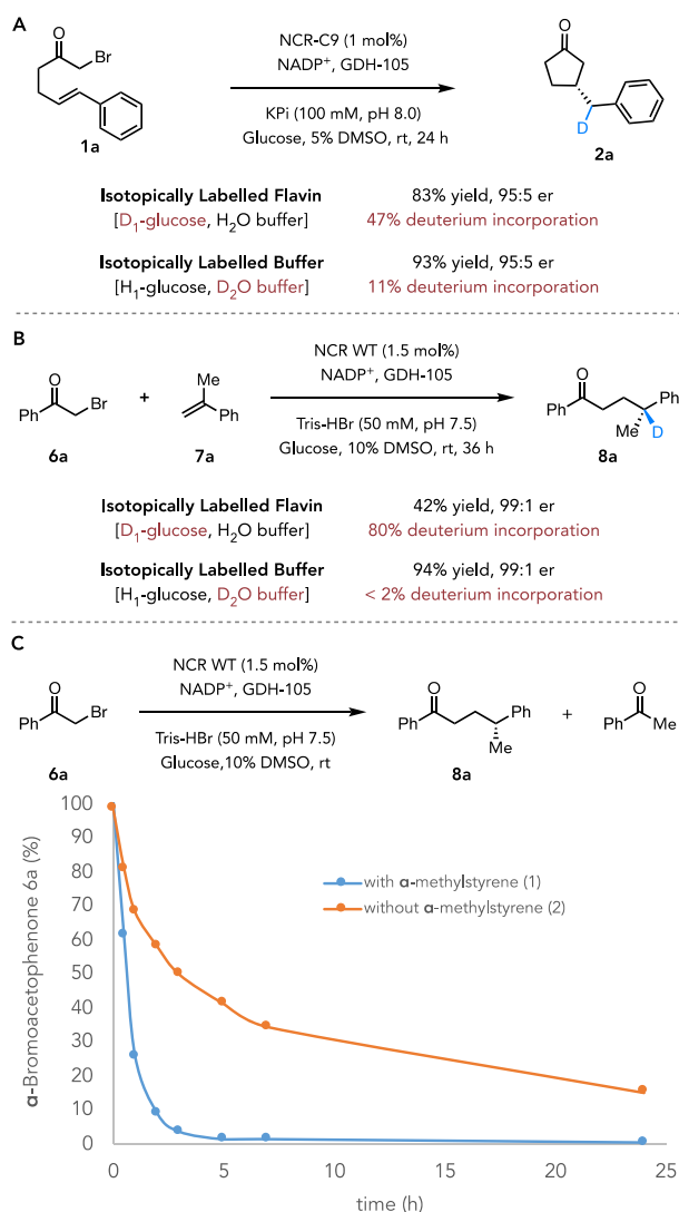
Figure 3. Deuterium labeling experiments. (A) Deuterium labeling experiments for the cyclization mediated by NCR-C9. (B) Deuterium labeling experiments for the intermolecular hydroalkylation catalyzed by wild-type NCR. (C) \alpha -Methylstyrene ( 7a ) affects the depletion of \alpha -bromoacetophenone ( 6a ) in NCR-catalyzed reaction. For experimental details, see SI Figures 6–15.
