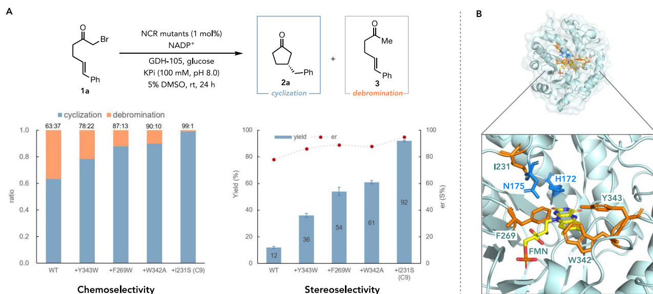
Figure 2. Directed evolution of NCR catalysts for non-natural asymmetric radical cyclization. (A) Chemoselectivity (cyclization versus debrominative hydrogenation), stereoselectivity, and yields improvement of NCR variants over wild-type NCR. Standard reaction conditions: the reaction mixture (500 \mu L) consisted of model substrate ( 1a , 0.004 mmol), GDH-105 (0.5 mg), glucose (5.0 mg), NADP + (0.5 mg), and purified NCR variants (1.0 mol %) in buffer (100 mM KPi buffer pH 8.0) with 5% DMSO as cosolvent at room temperature for 24 h. Yields were determined via HPLC relative to an internal standard (average of triplicate). Enantiomeric ratio (er) was determined via HPLC on a chiral stationary phase. (B) Crystal structure of wild-type NCR (PDB: 4s3u). Residues for substrate binding (H172 and N175) are shown as blue sticks. Four beneficial sites Y343, F269, W342, and I231 are shown in orange sticks.
