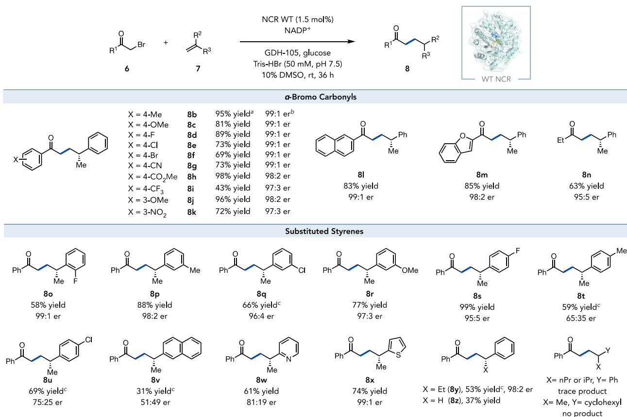
Scheme 2. Asymmetric Intermolecular Radical Hydroalkylation Catalyzed by Wild-Type NCR d
