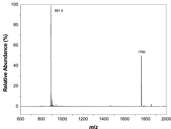
FIGURE 8. ESI mass spectrum of N -linked peptidoresorc[4]arene 10 (positive ion mode).
