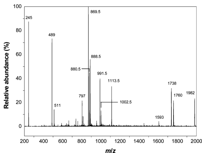
FIGURE 10. ESI mass spectrum of a 1:7 molar ratio solution of resorc[4]arene 10 and dipeptide 6 .
