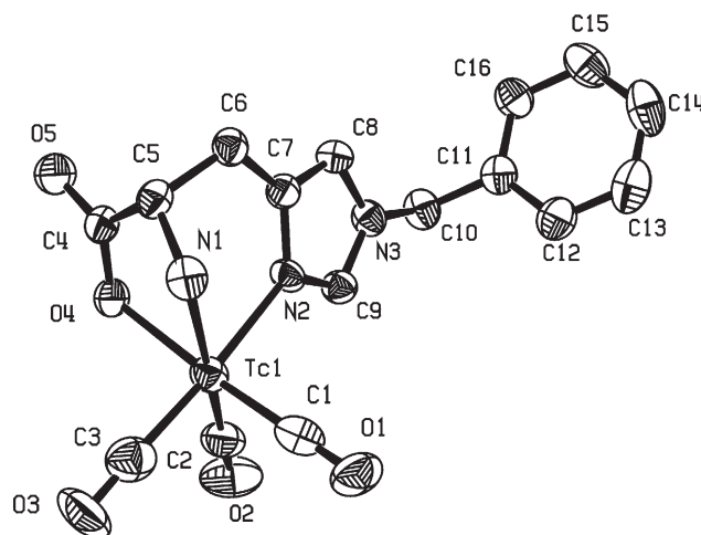
Fig. 1 ORTEP projection of Tc(His-N ε -benzyl)(CO) 3 ·H 2 O at 50% probability level. Hydrogen atoms as well as the H 2 O molecule are omitted for clarity. Selected bond lengths (Å): Tc(1)–C(1) 1.895(6), Tc(1)–C(2) 1.916(5), Tc(1)–C(3) 1.929(5), Tc(1)–O(4) 2.165(3), Tc(1)–N(1) 2.200(3), Tc(1)–N(2) 2.204(3).
