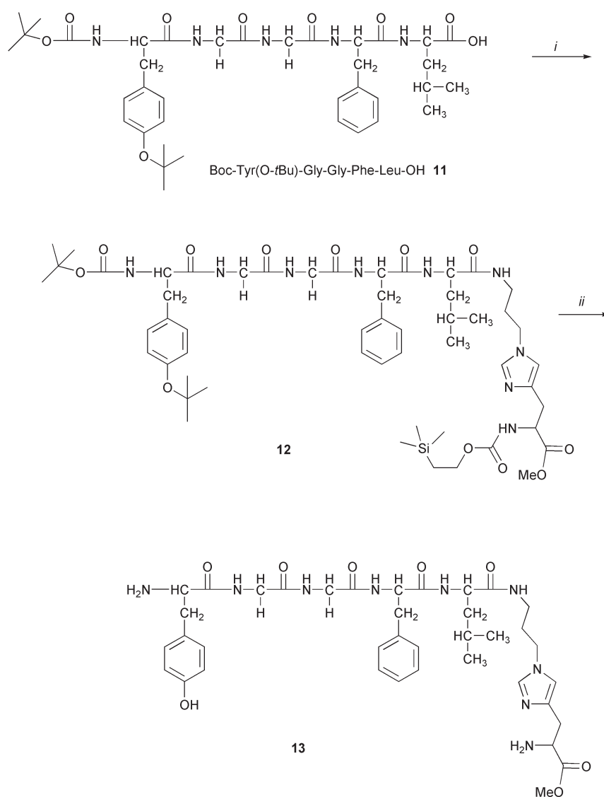
Scheme 5 Reagents and conditions: i) 8 , DMF, \text{HNEt}_3 , TBTU, RT, 49%; ii) TFA, \text{CH}_2\text{Cl}_2 , RT, 88%.
