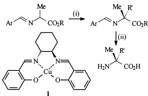
Scheme 1. Reagents and conditions: (i) NaOH/R'X/ 1 (2 mol%), toluene, rt; (ii) H 3 O + .
