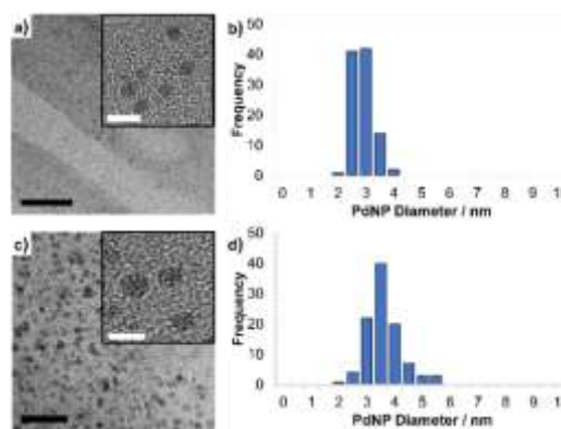
Figure 3 HRTEM images of (a) 3a and (c) 3a-PEG generated in-situ , and (b) and (d) corresponding particle size distributions determined by counting >100 particles. Mean nanoparticle diameters are 2.61 \pm 0.38 nm and 3.36 \pm 0.61 nm for 3a and 3a-PEG formed in-situ , respectively. Black and white scale bars are 25 and 10 nm, respectively.
