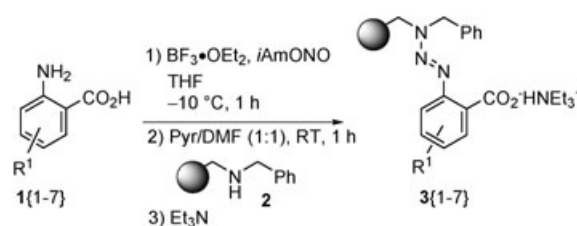
Scheme 2. Synthesis of the triazene resins 3 .
