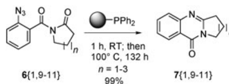
Scheme 8. Synthesis of deoxyvasicinone ( 7 {1,9}) and related heterocycles.
