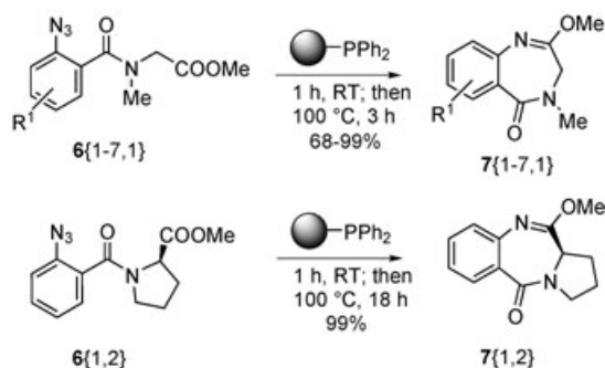
Scheme 5. Intramolecular aza-Wittig reaction.
