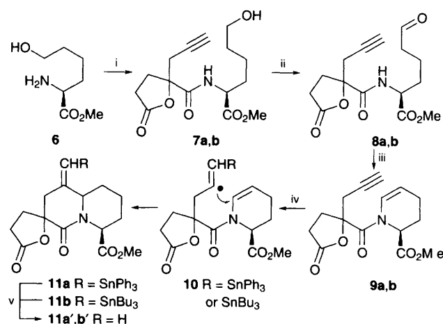
Scheme 2 Reagents and conditions: i, 6 , DMF, N -methyl morpholine, 1-hydroxybenzotriazole 5 , 1-(3-dimethylaminopropyl)-3-ethylcarbodiimide, room temp., 12 h, 65%; ii, PCC, 4   molecular sieves, CH 2 Cl 2 , room temp., 1.5 h, 73% for 8a , 87% for 8b ; iii, TFA, 4   molecular sieves, CH 2 Cl 2 , room temp., 4 h for 8a , and 1 h for 8b , 82% for 8a , 65% for 8b ; iv, Ph 3 SnH, AIBN, PhMe, reflux for 8a , Bu 3 SnH, AIBN, PhMe, reflux for 8b ; v, TFA, THF, 12 h at room temp., 2 h at 60  C for 9a , TFA, THF, 5 h at room temperature for 9b , 62% overall for 11a' and 89% overall for 11b'
