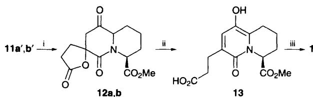
Scheme 3 Reagents and conditions: i, O 3 , CH 2 Cl 2 , -78 °C, Ph 3 P, -78 °C to room temp; ii, Et 3 N, THF, 60 °C, 2 h, 63% overall for each isomer; iii, (Bu 3 Sn) 2 O, PhH, reflux, 3 d, 67%
