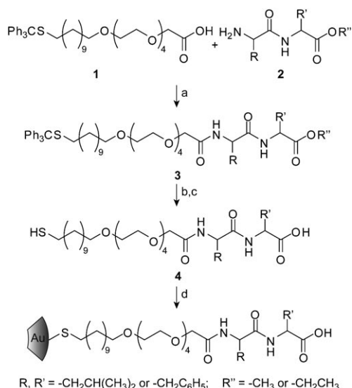
Scheme 1. Synthesis of dipeptide-functionalized thiol ligands and fabrication of the corresponding gold NPs: a) EDC, HOBT, DIPEA, \text{CH}_2\text{Cl}_2 , RT, 36 h, 70%; b) LiOH, THF/ \text{H}_2\text{O} , RT, 2 h, 100%; c) TFA, TIPS, \text{CH}_2\text{Cl}_2 , RT, 12 h, 50–75%; d) \text{C}_5 -AuNP, \text{CH}_2\text{Cl}_2 , 2 d, quantitative.
