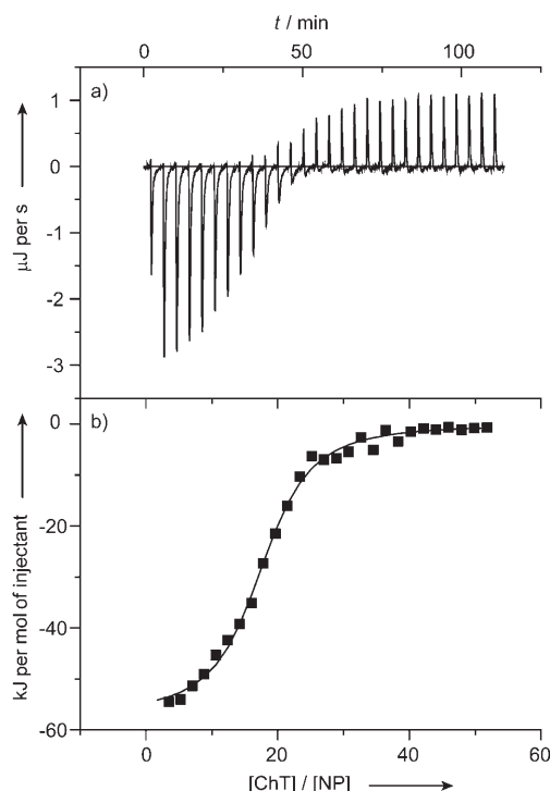
Figure 3. Isothermal titration calorimetry measuring the binding of ChT to NP_L-Phe-D-Phe: a) the heat change when ChT (400 \mu\text{M} ) is titrated into NP_L-Phe-D-Phe (2.5 \mu\text{M} ), and b) the integrated data (■) and the best fit to a nonlinear function with the assumption of a single type of binding sites (—).
