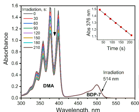
Figure 5. Photosensitized oxidation of 1,9-dimethylantracene in the presence of BDP-7 in air saturated acetonitrile solution irradiated with 514 nm laser ( 12 \text{ mW cm}^{-2} ). Inset: change of absorbance at 376 nm with time.
