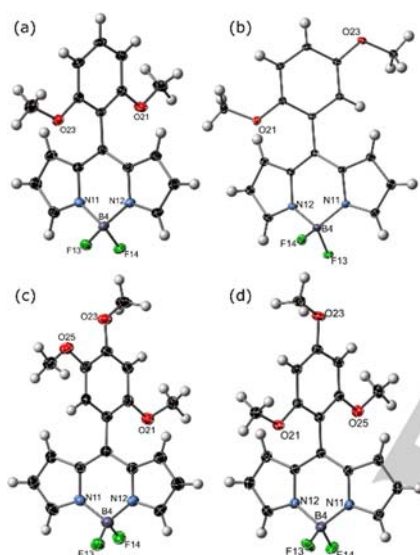
Figure 3. The individual molecular units of compound (a) BDP-4·½DCM (solvate omitted), (b) BDP-5 , (c) BDP-6 and (d) BDP-7 ; thermal ellipsoids are shown at the 50% probability level, H-atoms are represented as spheres of fixed radius.
