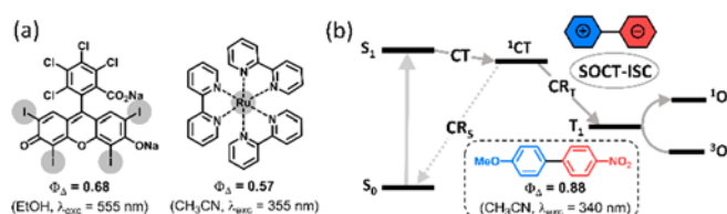
Figure 1. (a) Examples of heavy-atom-containing dyes. \Phi_{\Delta} – singlet oxygen quantum yield (solvent and excitation wavelength are given). (b) Jablonski diagram illustrating the formation of triplet excited state via the SOCT-ISC mechanism.
