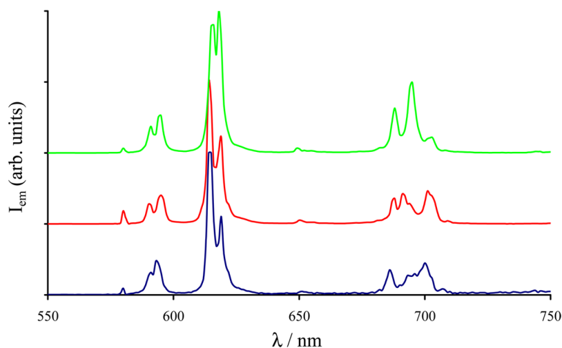
Figure 3. Emission spectra of the 1b , 6b , and 7b complexes (from bottom to top) in TRIS/HCl buffer (0.01 M, pH 7.4; \lambda_{\text{exc}} = 318\text{ nm} ).
