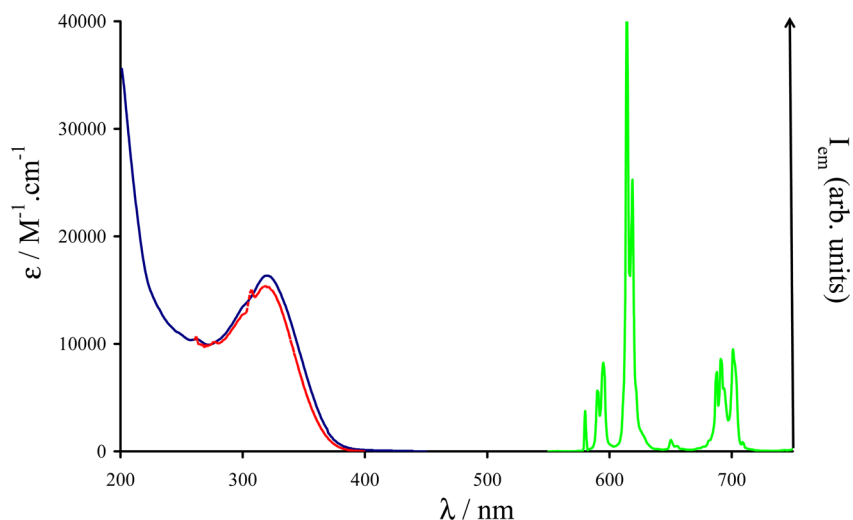
Figure 2. UV-vis absorption (blue), excitation ( \lambda_{\text{em}} = 615\text{ nm} , red) and emission ( \lambda_{\text{exc}} = 319\text{ nm} , green) spectra of 1b in 0.01 M TRIS/HCl buffer at pH 7.4.
