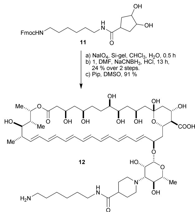
Scheme 2 Synthesis of diaminohehexyl pyridyl amphotericin B.
