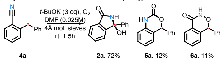
Scheme 21. C-H activation and cyclization of a nitrile substrate.
