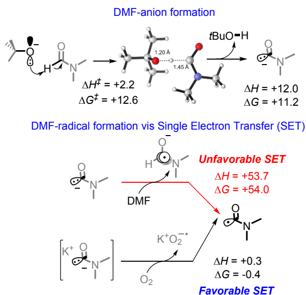
Scheme 7. Formation of DMF radical. All energies reported in kcal/mol.
