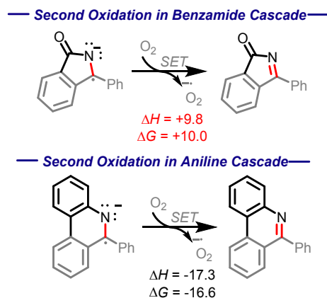
Scheme 13. Contrasting thermodynamics (kcal/mol) for the C=N forming oxidations in the amide and aniline cascades.
