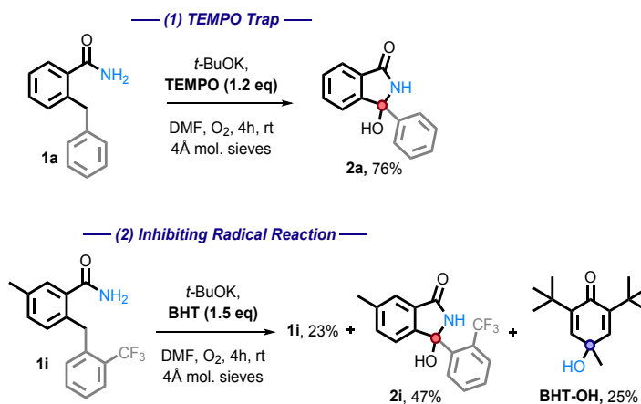
Scheme 14. Radical coupling mechanistic studies.
