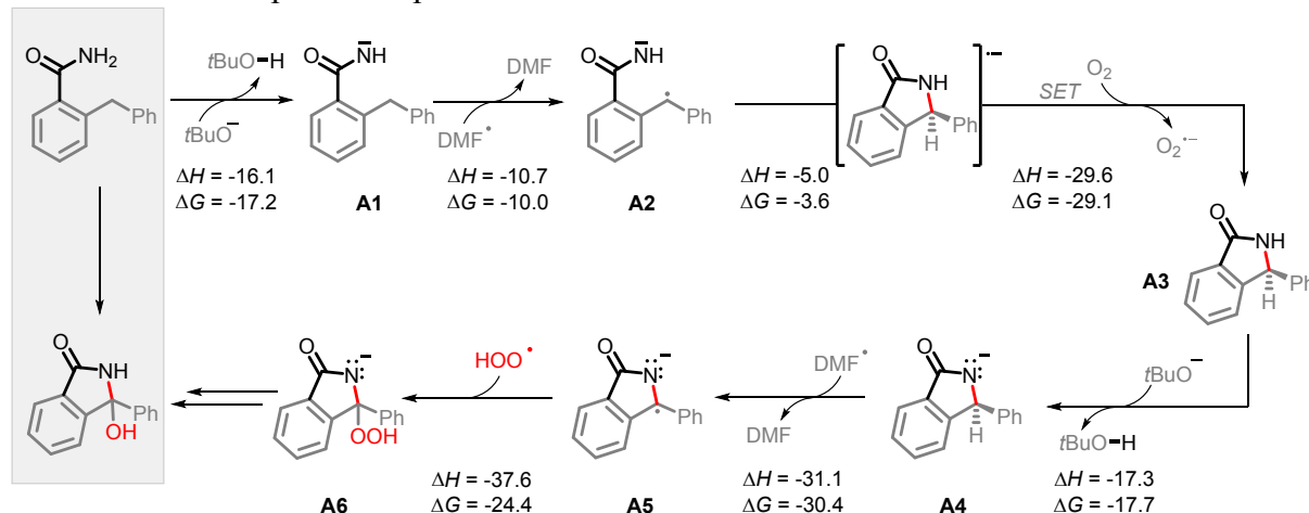
Scheme 6. Proposed mechanism and calculated reaction thermodynamics for the individual steps in the N-H/C-H amidation. All energies are in kcal/mol.
