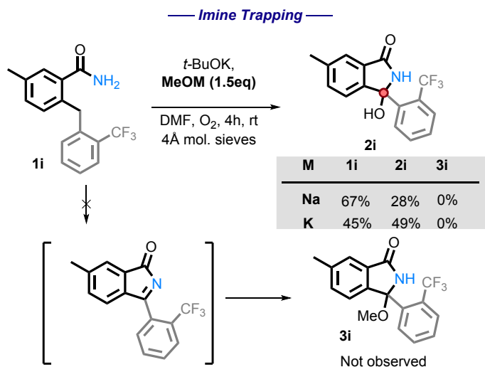
Scheme 12. Attempting to trap the hypothetical imine intermediate.
