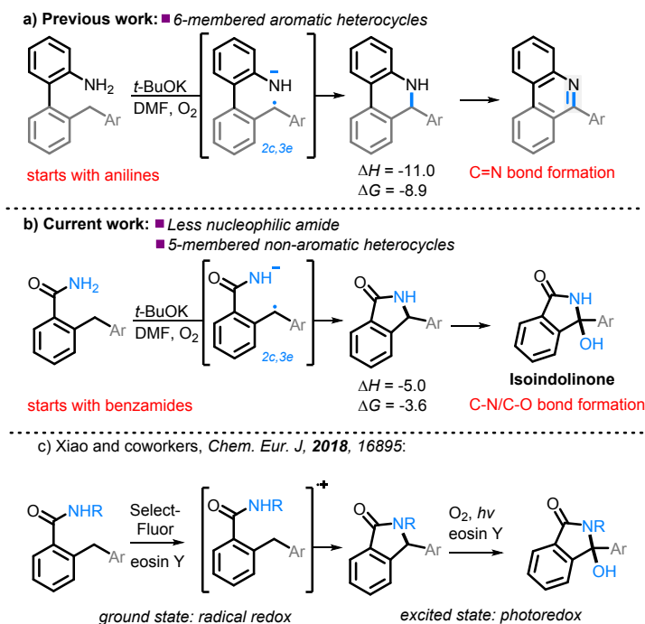
Scheme 3. Expanding previous work to utilize less nucleophilic amides, as well as the formation of non-aromatic five membered heterocycles, and C-N/C-O bond formation. All energies are in kcal/mol.
