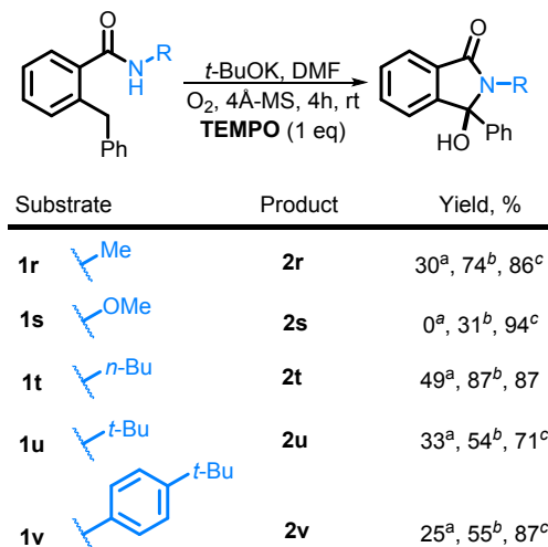
Scheme 20. Improved C-H activation with TEMPO as an additive. Reaction conditions: Secondary benzamide (0.025 M), t\text{-BuOK} (3 eq), DMF (2 mL), 4Å MS, \text{O}_2 balloon, reactions stirred at r.t. overnight. (a) Isolated yields for reaction performed under standard conditions. (b) Isolated yields for reactions with the addition of TEMPO. (c) Yields based of reclaimed starting materials with the addition TEMPO.
