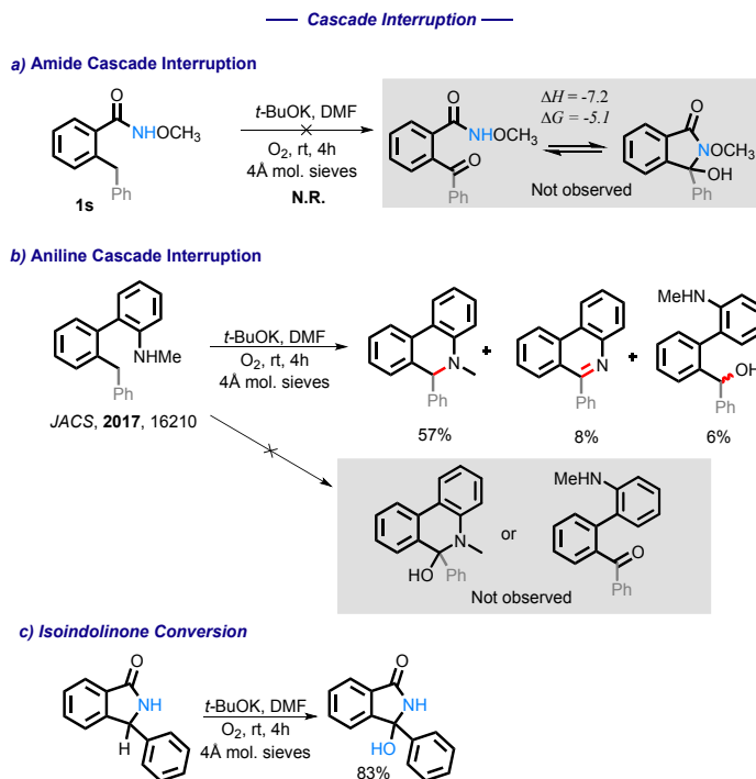
Scheme 5. Interruption of the amide and aniline cascades
