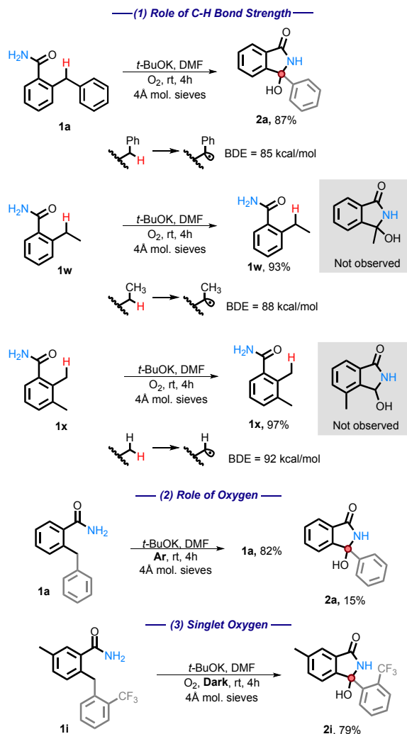
Scheme 4: Mechanistic tests for the C-H bond strength and for the participation of oxygen. All energies are reported in kcal/mol.
