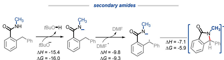
Scheme 17. Calculations for the deprotonation, HAT, and radical-anion cyclization of 1r . All energies are reported in kcal/mol.
