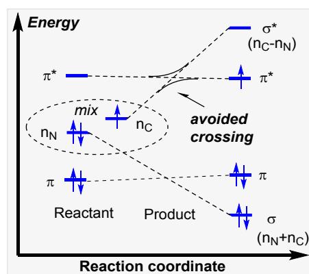
Scheme 10. State crossing avoids populating the high energy \sigma^*_{\text{C-N}} orbital.
