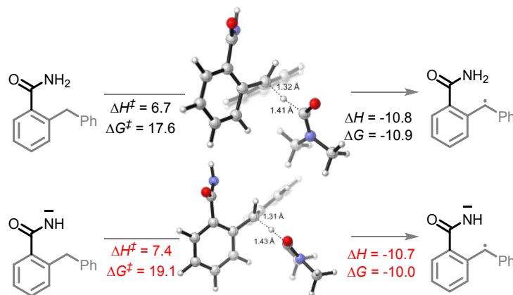
Scheme 8. Reaction energy profiles and twisted transition states for C-H activation in neutral and deprotonated substrates. All energies are in kcal/mol.
