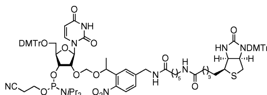
structure of phosphoramidite for a rapid RNA synthesis
