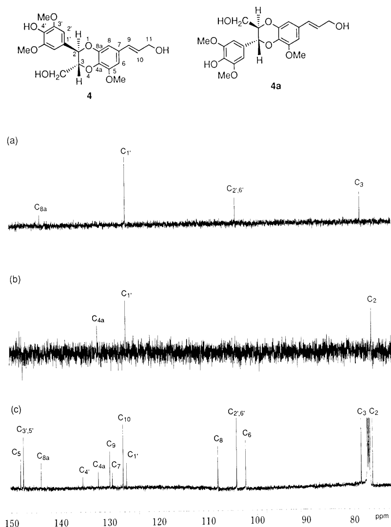
Fig. 1. The Selective INEPT Experiment for Nitidanin ( 4 )
