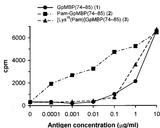
Figure 2. Proliferative response of a TCL generated from spleen cells of Lewis rats immunized with MBP to different concentrations of the wild-type peptide 1 and its lipoderivatives 2 and 3 . Data show a representative experiment out of three carried out with different TCLs, and they are expressed as cpm. Background proliferation was 315 cpm.
