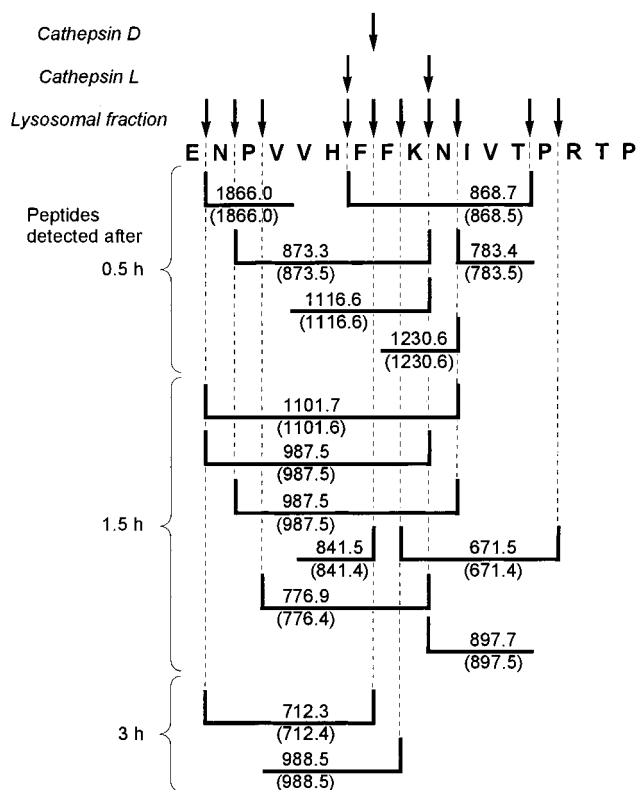
Figure 6. Cathepsin D and L and lysosomal fraction cleavage sites (h) of GpMBP(82–98) and fragments generated by digestion with lysosomal fraction, as detected by LC-MS analysis ( [M + H]^+ found; calculated values in parentheses).
