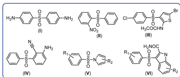
Fig. 1 The structures of dapsone (I), 2-nitrophenyl phenyl sulfone (II), N -(5-bromo-3-((4-chlorophenyl)sulfonyl)thiophen-2-yl)acetamide (III), 2-amino-6-arylsulfonylbenzonitrile (IV), pyrrolarylsulfone (V) and indolylaryl sulfones (VI).
