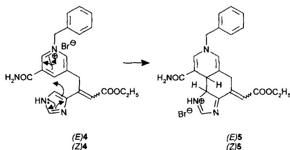
Scheme 3. Model for the urocanase reaction.
