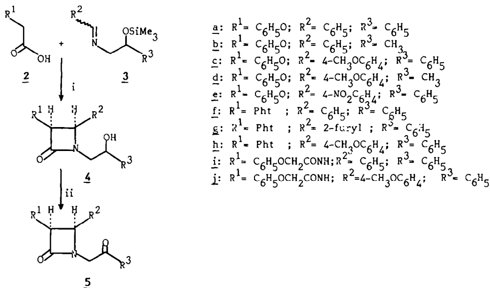
Scheme 1. Reagents and Conditions : i , \text{PhO}(\text{PO})\text{Cl}_2, \text{NEt}_3, \text{Cl}_2\text{CH}_2 , r.t., ref.10; ii , NDC(2.5 equiv.), pyridine (20 equiv.), \text{Cl}_2\text{CH}_2 , r.t.
