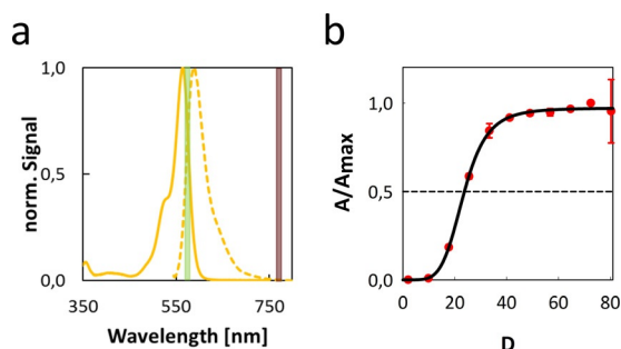
Figure 1. a) Normalized absorption (solid line) and emission (dashed line) spectra of pyridine-containing rhodamine 5-H (565pR) in PBS at pH 7.5. Green bar shows excitation at 561 nm and red bar represent 775 nm STED laser. b) Normalized absorption ( A/A_{\max} ) at \lambda_{\max} of 5-H (565pR) plotted vs. dielectric constant ( D ) of dioxane-water mixtures. D_{0.5} values (Table 1) correspond to the intersection of interpolated graphs with A/A_{\max} = 0.5 line.
