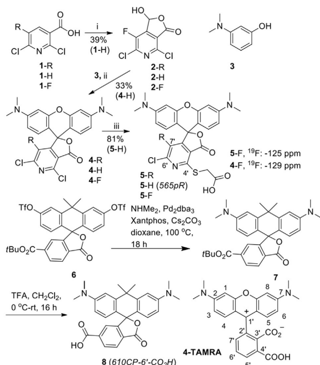
Scheme 2. Synthesis of chloropyridine-containing rhodamine dyes 5-R as analogs of 4-TAMRA (with the uniform numeration of the carbon atoms). Reagents and conditions: i) LDA, THF, -78^{\circ}\text{C} , 1 h; then DMF, -78^{\circ}\text{C} to RT, 1 h; ii) 1,2-dichlorobenzene, 120^{\circ}\text{C} , 3 h; iii) HSCo 2 H, Et 3 N, DMF, RT, 1 h.
