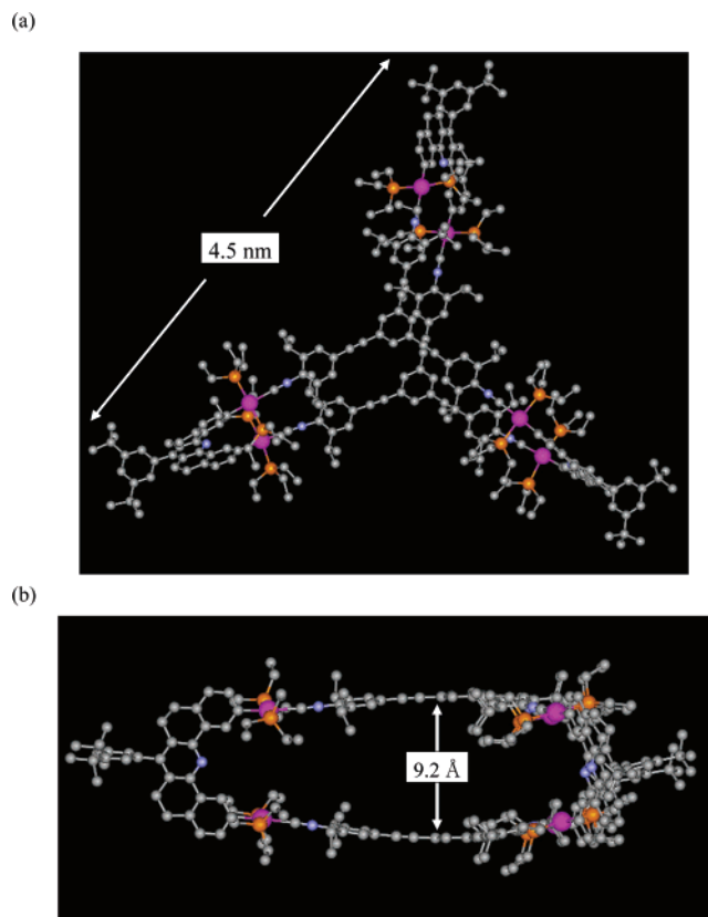
Figure 4. Ab initio calculation of optimized trigonal prism 11 : (a) overall figure; (b) side view for 11 . The molecule seems to have a C_3 symmetry or a modified C_{3h} symmetry. H atoms are omitted for clarity.
