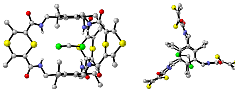
Figure 2. Side (left) and top (right) views of the crystal structure of Receptor 3 with CH 2 Cl 2 as a solvate. C–H hydrogens are omitted for clarity.
