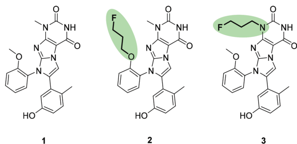
Scheme 2 Literature known lead compound 1 and proposed structures of fluorine-containing-compounds 2 and 3 with highlighted labelling positions.
