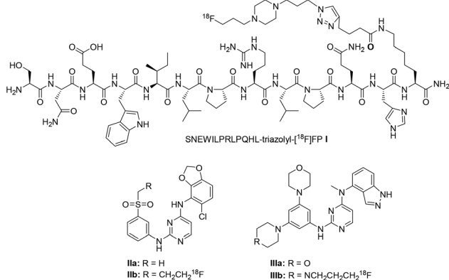
Scheme 1 Structures of ^{11}\text{C} - and ^{18}\text{F} -labelled radiotracers I–III based on Eph inhibitors prepared by our group.
