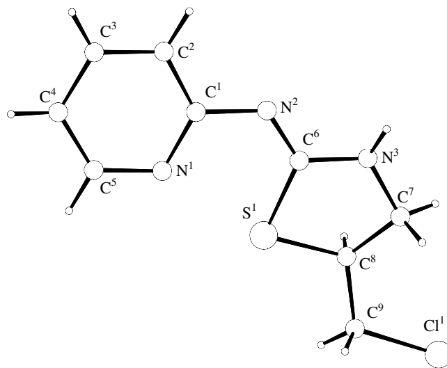
Fig. 1. Structure of the molecule of N -(5-chloromethyl-1,3-thiazolidin-2-ylidene)pyridin-2-amine ( III ) according to the X-ray diffraction data. Principal bond lengths (Å) and bond angles (deg): \text{C}^1\text{--N}^2 1.397(5), \text{N}^2\text{--C}^6 1.299(6), \text{N}^3\text{--C}^6 1.330(5), \text{N}^3\text{--C}^7 1.435(6), \text{S}^1\text{--C}^6 1.767(5), \text{S}^1\text{--C}^8 1.825(5), \text{C}^7\text{--C}^8 1.487(7); \text{C}^6\text{S}^1\text{C}^8 90.9(2), \text{C}^1\text{N}^2\text{C}^6 122.0(4), \text{C}^6\text{N}^3\text{C}^7 117.6(4).
