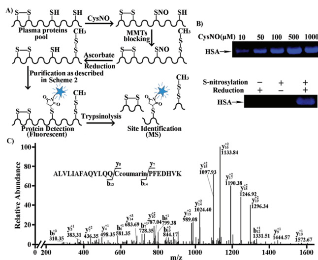
Figure 4. (A) Schematic of the protocol for identifying protein Cys–SNO modification using phototrigger 1_L and 1_{UL} . (B) Top: Fluorescence imaging of the SDS-PAGE of human plasma proteins treated with various concentrations of CysNO (1, 0 \mu\text{M} ; 2, 10 \mu\text{M} ; 3, 50 \mu\text{M} ; 4, 100 \mu\text{M} ; 5, 500 \mu\text{M} ; 6, 1000 \mu\text{M} ) and purified by affinity capture followed by photolysis. Bottom: Fluorescence imaging of the SDS-PAGE of the S-nitrosylated plasma protein under different control conditions. (C) Tandem MS/MS spectra of the extracted ion on the [M + H]^+ peak ( m/z 926.1 in Figure S8) of peptides T21–41 in HSA with the unique coumarin adduct.
