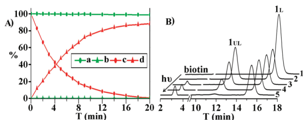
Figure 1. (A) Photolysis monitored by HPLC: (a) consumption curve of 1_L ; (b) release curve of biotin from 1_L ; (c) consumption curve of 1_{UL} ; (d) release curve of biotin from 1_{UL} . (B) HPLC profiles of 1_L : (1) 1_L alone; (2) mixture of 1_L and 1_{UL} by partial thiol activation of 1_L ; (3–5) photolysis of the mixture in (2) for (3) 3, (4) 8, and (5) 18 min.
