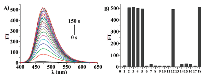
Figure 2. (A) The presence of 100 \mu M \beta -mercaptoethanol in the 10 \mu M 1_L solution of 6:4 MeOH/tris-HCl buffer (pH 7.4) gradually converted 1_L to 1_{UL} , thus enhancing the fluorescence intensity at 480 nm ( \lambda_{ex} = 390 nm). (B) Responses of 10 \mu M 1_L upon exposure to different analytes (100 \mu M) in 6:4 solutions of MeOH or DMSO (for proteins) and Tris-HCl buffer (pH 7.4). The thiol-bearing analytes could unlock 1_L and thus produce strong luminescence, whereas solutions of those that could not unlock 1_L remained dark: 1, blank; 2, \beta -mercaptoethanol; 3, cysteine; 4, homocysteine; 5, glutathione; 6, glutamic acid, phenylalanine, alanine; 7, lysine; 8, glucose; 9, ascorbate; 10, H_2O_2 ; 11, Mg^{2+} , Fe^{3+} , Zn^{2+} , Ca^{2+} ; 12, BSA; 13, BSA + NEM; 14, transferrin; 15, ovalbumin; 16, trypsin inhibitor; 17, lysozyme; 18, lysozyme + TCEP.
