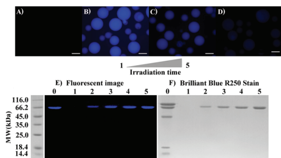
Figure 3. Photolysis of streptavidin agarose beads to release the captured biotinylated protein using visible-light irradiation (CHF-XM-500w lamp, >400 \text{ nm} filter, 60 \text{ mW/cm}^2 ). (top) fluorescence microscope images of photolyzed beads: (A) blank beads, (B–D) protein-loaded beads after 0, 2, and 8 min of light exposure. (bottom) SDS-PAGE of the supernatant viewed via (E) fluorescence or (F) Coomassie brilliant blue R250 stain: lane 0 contained the original protein mixtures incubated with 1_L before affinity capture, whereas lanes 1–5 were loaded with the supernatant after different light exposure times (1, 0 min; 2, 1 min; 3, 2 min; 4, 4 min; 5, 8 min).
