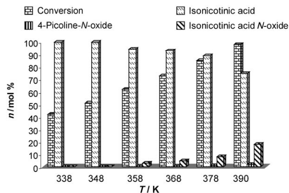
Figure 2. The effect of temperature in the catalytic, solvent-free oxidation of 4-picoline using \text{Mn}^{\text{III}}\text{AlPO-5} as the catalyst.
