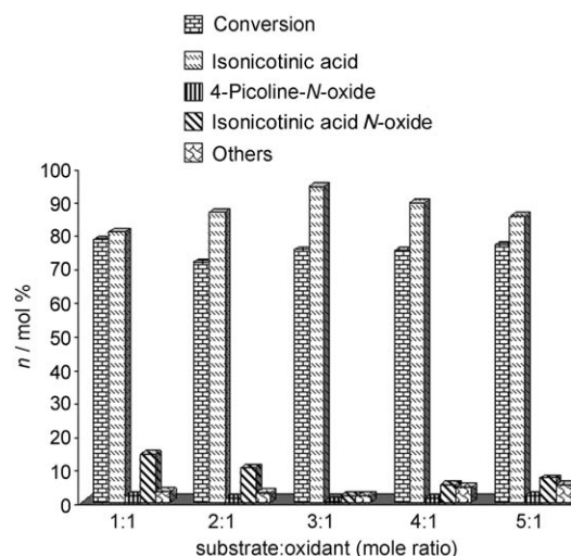
Figure 4. The influence of substrate:oxidant mole ratios, showing that an optimal ratio is required for enhancing the activity and selectivity, in the oxidation of 4-picoline after 4 h at 368 K.
