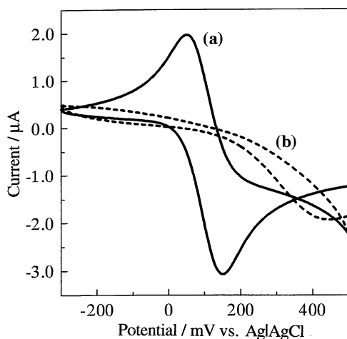
Figure 2. Cyclic voltammograms of 1.0 mM potassium ferrocyanide at NutraAvidin-SAM electrode in: a) 0.1 M acetate buffer (pH 4.0). b) 0.1 M phosphate buffer (pH 7.0). Scan rate 50 mV/s.
