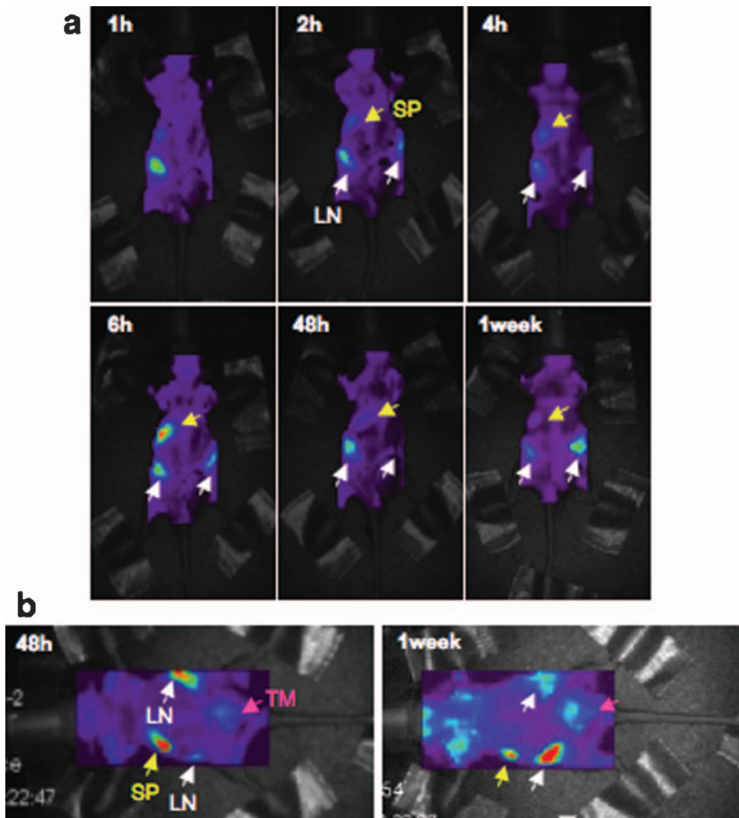
Figure 3: Fluorescence imaging of lymphocytes in mice. Labeled and/or engineered cells were administrated intravenously ( n = 3 , 100 \mu\text{L}/\text{mouse} , 10^4 cells) and the whole body was scanned from the back side by eXplore Optix, GE Healthcare, Bioscience (excitation at 646 nm, emission 663 nm), 1 h, 2 h, 4 h, 6 h, 48 h, and 1 week after injection. Data were normalized. SP: spleen; LN: lymph node of epidermal intestinal tract; TM: DLD-1 human colon carcinoma. (a) Cy5-labeled cells injected to nude mice that were implanted with DLD-1 at the dorsal division; (b) both Cy5-labeled and N -glycan-engineered lymphocytes in the tumor model. (Figure available in color online.)
