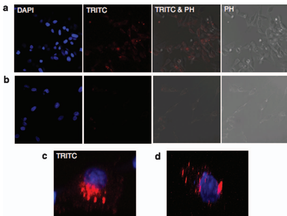
Figure 2: Confocal microscopy of biotin- and N -glycan-modified C6 glioma cells (DAPI-, TRITC-, and PH detections). (a) 1b -Modified cell on TRITC-avidin treatments; (b) control cell treated with biotin-containing phosphine 3 on TRITC-avidin treatments; (c) 1c -modified cell on SNA lectin (Neu \alpha (2,6)Gal-specific) treatments; (d) intact cell on SNA lectin treatments. PH: phase contrast. (Figure available in color online.)
