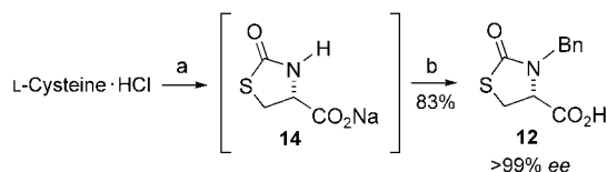
Scheme 3. One-pot synthesis of 12 from L-cysteine. Reagents and conditions: a) ClCO 2 Ph, NaOH, H 2 O, toluene, 25°C, 2 h; b) to the aqueous phase were added BnCl, NaOH, DMSO, H 2 O, 25°C, 15 h.
