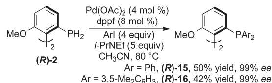
Scheme 3. Synthesis of MeOBIPHEP Analogues
