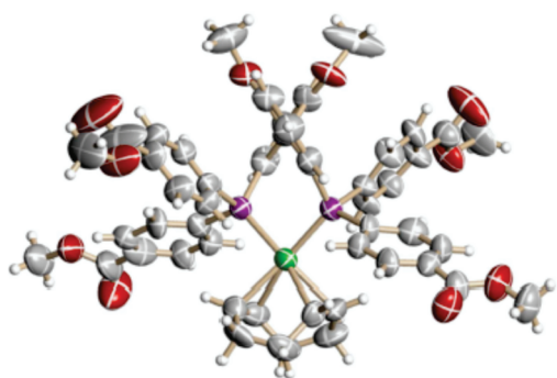
Figure 1. X-ray structure of [\text{Rh}((\text{S})\text{-3})(\text{cod})]\text{BF}_4 complex.
