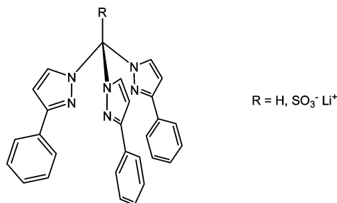
Figure 1. Schematic structures of the tris(3-phenylpyrazolyl)methane compounds \text{Tpm}^{\text{Ph}} ( \text{R} = \text{H} ) and \text{Li}(\text{Tpms}^{\text{Ph}}) ( \text{R} = \text{SO}_3\text{Li} ).
