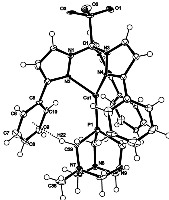
Figure 5. ORTEP plot of [\text{Cu}(\text{Tpms}^{\text{Ph}})(\text{mPTA})][\text{PF}_6] ( 5 ), with ellipsoids shown at 50% probability; hydrogen atoms are shown but the [\text{PF}_6]^- counterion and one molecule of crystallization acetone are omitted for clarity. The dashed line indicates the C–H... \pi intramolecular (2.489 Å) interaction between C(29)–H(22) and the \pi -phenyl ring (C(5) to C(10)).
