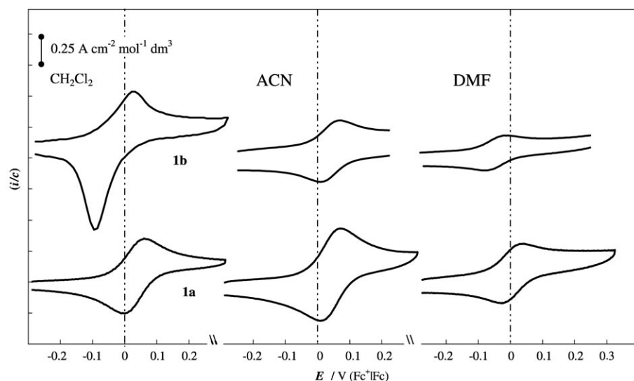
Figure 2. Comparison of the CV patterns obtained at \nu = 0.2 \text{ V s}^{-1} in the three organic solvents \text{CH}_2\text{Cl}_2 , MeCN and DMF, for the monofluorene-labelled ester 1a and acid 1b .
