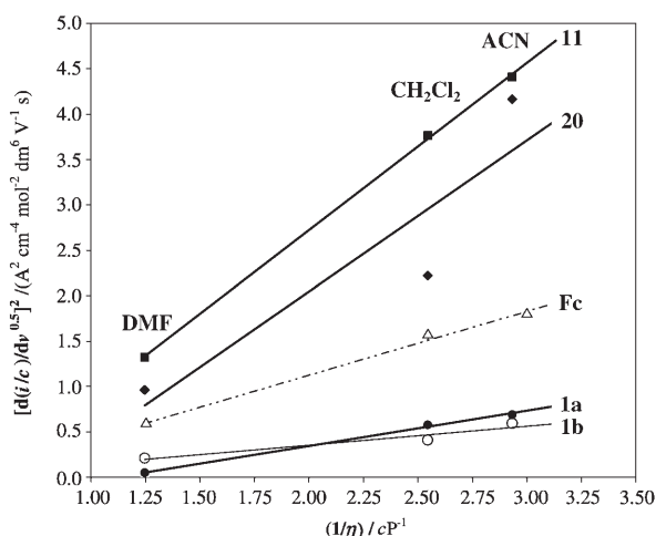
Figure 3. Squared slopes of the normalised current versus \nu^{0.5} linear characteristics, plotted against the reciprocal of solvent viscosity \eta (verification of Stokes' law): the reference ferrocene compound ( \blacktriangle ); the monofluorene-labelled ester and acid, 1a ( \bullet ) and 1b ( \circ ); and the trifluorene-labelled esters 11 ( \blacksquare ) and 20 ( \blacklozenge ).
