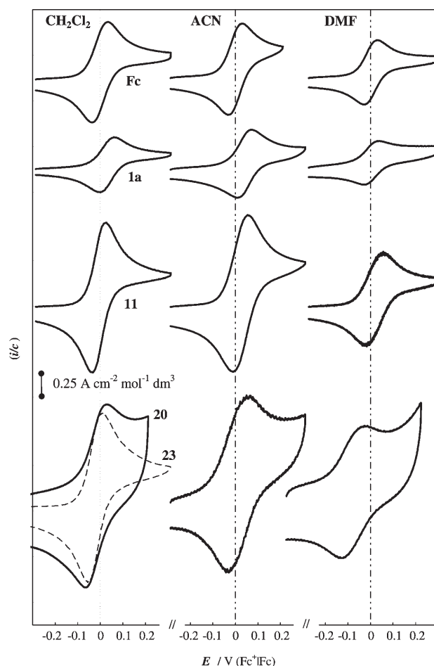
Figure 1. A synopsis of the CV patterns obtained at \nu = 0.2 \text{ V s}^{-1} for the four ester substrates 1a , 11 , 20 and 23 in the three organic solvents CH 2 Cl 2 , MeCN and DMF, with ferrocene as a reference.
