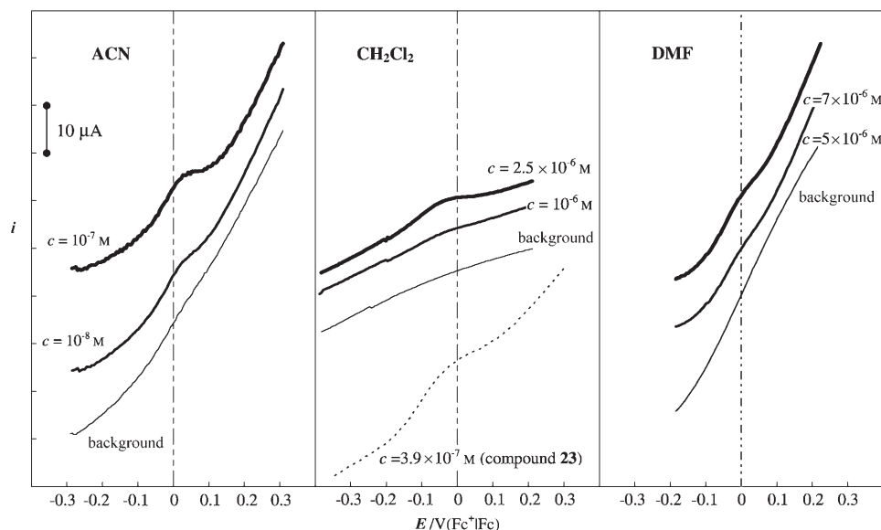
Figure 4. DPV patterns obtained by working with very low concentrations ( c ) of the Tris-ferrocene-labelled esters 11 in the three organic solvents \text{CH}_2\text{Cl}_2 , MeCN, DMF and 23 in \text{CH}_2\text{Cl}_2 (dotted line) for the evaluation of the relevant detection limits.
