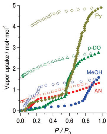
Figure 13. Adsorption isotherms obtained for acetoneitrile (red square), methanol (blue circle), 1,4-dioxane (green triangle), and pyridine (yellow diamond) vapor in 8 . Closed and open symbols represent the adsorption and desorption processes, respectively.
