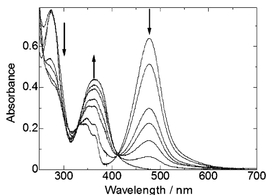
Figure 4. Changes in the absorption of 1 in acetonitrile upon addition of 70% aq. \text{HClO}_4 . Spectra were acquired for 0, 0.25, 0.5, 0.60, 0.70, 0.80, 1.00, and 1.20 equiv additions of acid.
