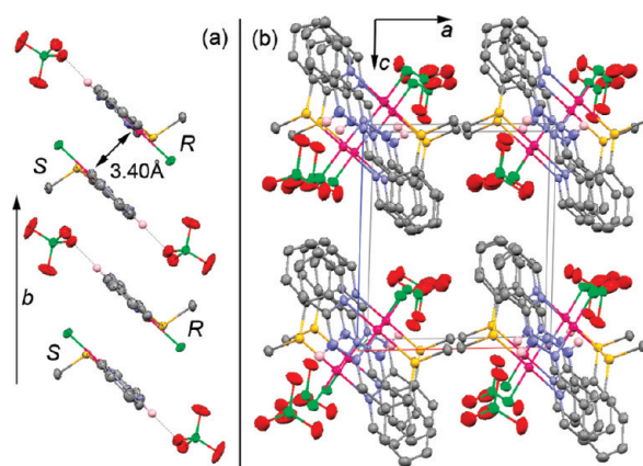
Figure 3. (a) Stacking structure and (b) packing diagram of 1H along the b axis with thermal vibrational ellipsoids at the 50% probability level. Dotted lines show hydrogen bonds. Carbon-bound hydrogen atoms are omitted for clarity.
