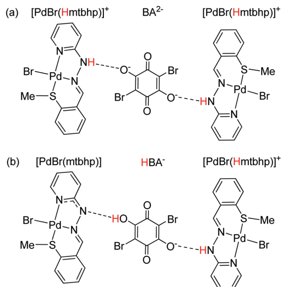
Scheme 1. Schematic Representation of Proton Transfer in HBPT Assembly 6 a
