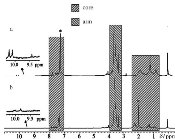
Figure 4. ^1\text{H} NMR spectra of HCP- star -PEG in a) \text{CDCl}_3 , and b) \text{CD}_3\text{CN} (400 MHz, 20 °C; the solvent peak is marked with an asterisk).
