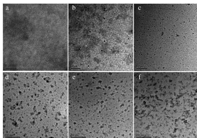
Figure 6. TEM photographs of HCP- star -PEG micelles in mixed solutions of chloroform and acetonitrile, the content of acetonitrile is as follows: a) 0, b) 20, c) 40, d) 60, e) 80, and f) 100 %. The scale bars represent 50 nm for a and b, and 200 nm for c–f.
