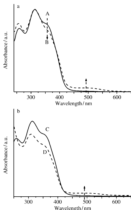
Figure 3. UV/Vis spectra of 3.8 \times 10^{-5} M solutions of a) HCP- star -PEG (A) and HCP- star -PEG with 2 \mu L TFA (B) and b) HCP- star -PEG (C) and HCP- star -PEG with 2 mg \text{SnCl}_2 (D) in chloroform.
