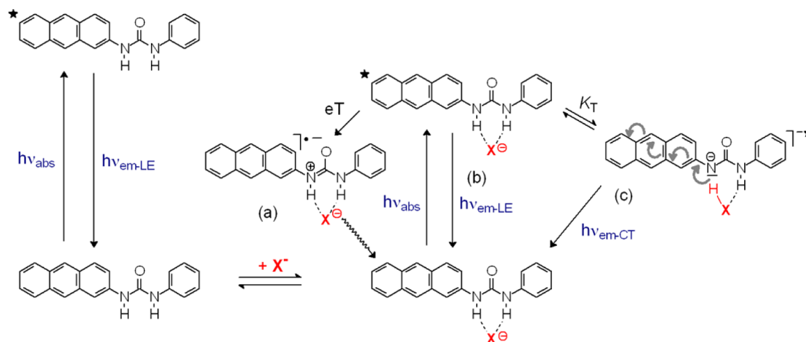
Figure 5. A qualitative sketch of the emissive behavior of the [L^1H \cdots X]^- complex. Route (a): X^- = CH_3COO^- , F^- in MeCN, quenching of the locally excited (LE) complex [*L^1H \cdots X]^- by eT from the partially negatively charged carbonyl oxygen atom. Route (b) X^- = Cl^- , Br^- : emission of the LE complex [*L^1H \cdots X]^- (red-shifted with respect to the uncomplexed receptor *L^1H ). Route (c): X^- = F^- , CH_3COO^- in DMSO. Charge transfer (CT) emission of the excited tautomeric complex originated from the proton transfer from one N-H fragment to X^- ; \pi -delocalization over the anthracenyl subunit is purely indicative.
