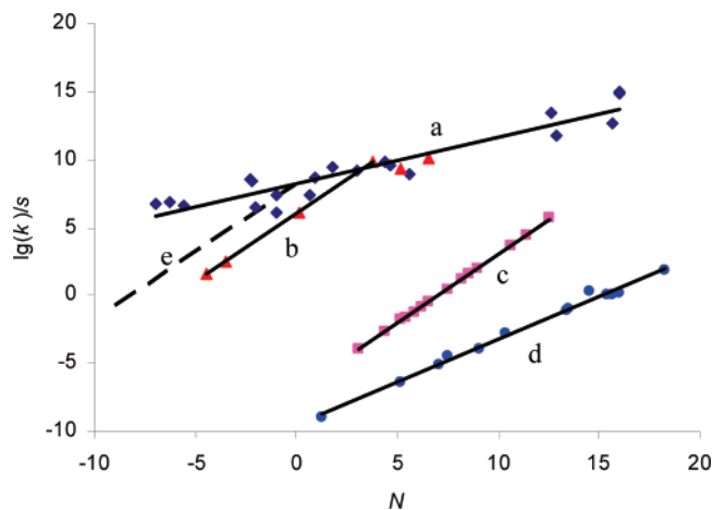
FIGURE 4. Dependence of (\log ^3k_{\text{NuH}})/s vs N for the reactions (a, \blacklozenge ) of 31 with the nucleophiles in Table 2 (except 21 and 29 ). Also reported literature data for the reactions of two benzhydryl cations, viz. (b, \blacktriangle ) (4\text{-ClC}_6\text{H}_4)_2\text{CH}^{+2a,e} and (c, \blacksquare ) (4\text{-Me}_2\text{NC}_6\text{H}_4)_2\text{CH}^{+2e} as well as of (d, \bullet ) S -methylidibenzothiophenium 1a with various nucleophiles. The broken line (e) corresponds to the equation (\log ^3k_{\text{NuH}})/s = 8.11 + N .
