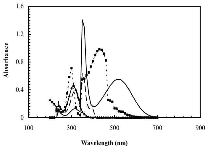
Fig. 2. Absorption spectra of TZ ( \blacktriangle ), reduced TZ (-----), CAA ( \blacksquare ) and the new CT complex between CAA and reduced TZ (____).
