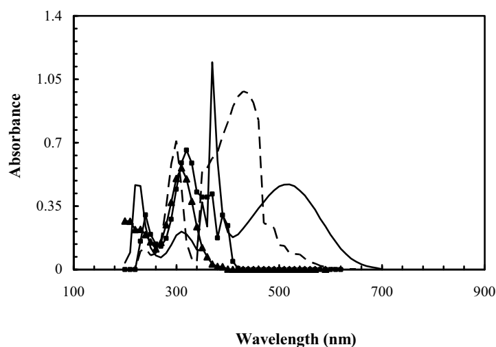
Fig. 1. Absorption spectra of MZ ( \blacktriangle ), reduced MZ ( \blacksquare ), CAA (-----) and the new CT complex between CAA and reduced MZ (____).
