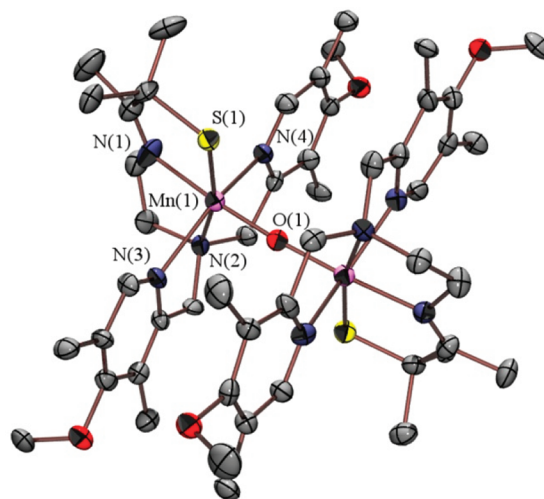
Figure 9. ORTEP diagram of \{[\text{Mn}^{\text{III}}(\text{S}^{\text{Me}_2}\text{N}_4(4\text{-MeO-3,5-Me}_2\text{-DPEN}))_2-(\mu\text{-O})]^{2+} \text{ with counterions, solvents of crystallization, and hydrogen atoms omitted. Selected distances (\AA) and angles (degrees): Mn–O(1)}_{\text{ave}} 1.75(1); \text{Mn–S(1)}_{\text{ave}} 2.28(2); \text{Mn–N(1)}_{\text{ave}} 2.01(4); \text{Mn–N(2)}_{\text{ave}} 2.18(2); \text{Mn–N(3,4)}_{\text{ave}} 2.23(2); \text{Mn–O(1)–Mn}, 175.4(7).
