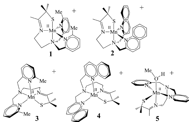
Figure 2. Chemdraw diagrams of [Mn II (S Me2 N 4 (6-Me-DPEN))]⁺ (1), [Mn II (S Me2 N 4 (2-QuinoEN))]⁺ (2), [Mn II (S Me2 N 4 (6-Me-DPPN))]⁺ (3), [Mn II (S Me2 N 4 (2-QuinoPN))]⁺ (4), and [Mn II (S Me2 N 4 (6-H-DPEN)(MeOH))]⁺ (5).
