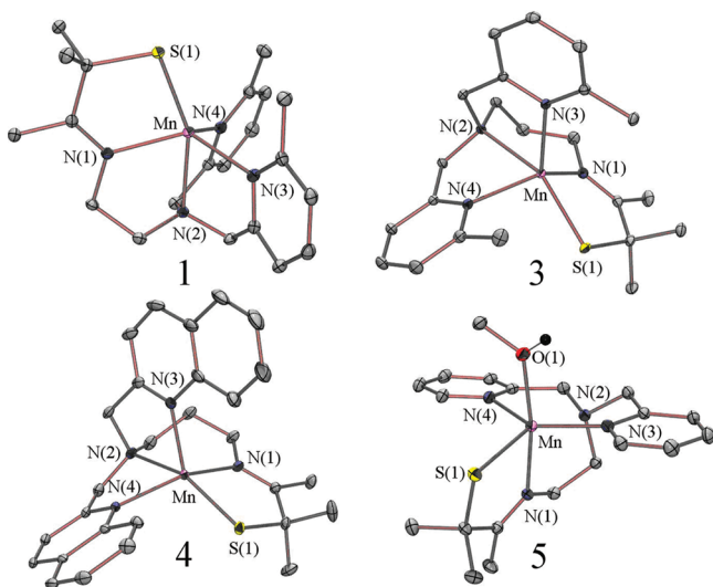
Figure 1. ORTEP diagrams of [Mn II (S Me2 N 4 (6-Me-DPEN))]⁺ (1), [Mn II (S Me2 N 4 (6-Me-DPPN))]⁺ (3), [Mn II (S Me2 N 4 (2-QuinoPN))]⁺ (4), and [Mn II (S Me2 N 4 (6-H-DPEN)(MeOH))]⁺ (5) with counterions, solvents of crystallization, and hydrogen atoms omitted.
