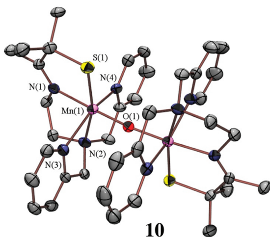
Figure 6. ORTEP diagram of \{[\text{Mn}^{\text{III}}(\text{S}^{\text{Me}_2}\text{N}_4(6\text{-H-DPEN)})]_2-(\mu\text{-O})\}^{2+} ( 10 ) with counterions, solvents of crystallization, and hydrogen atoms omitted.
