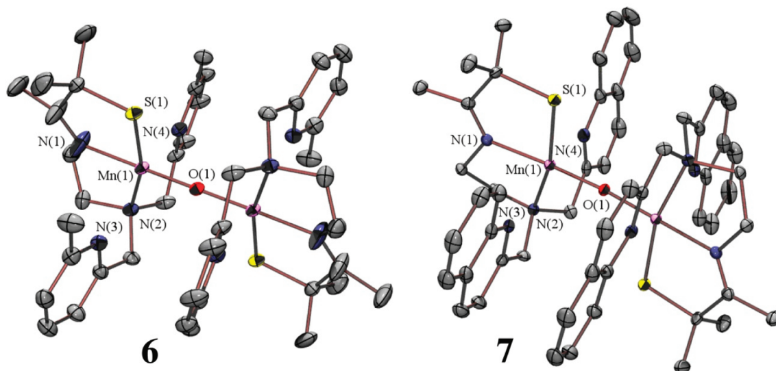
Figure 5. ORTEP diagrams of \{[\text{Mn}^{\text{III}}(\text{S}^{\text{Me}_2}\text{N}_4(6\text{-Me-DPEN)})]_2-(\mu\text{-O})\}^{2+} ( 6 ) and \{[\text{Mn}^{\text{III}}(\text{S}^{\text{Me}_2}\text{N}_4(\text{QuinoEN}))]_2-(\mu\text{-O})\}^{2+} ( 7 ) with counterions, solvents of crystallization, and hydrogen atoms omitted.
