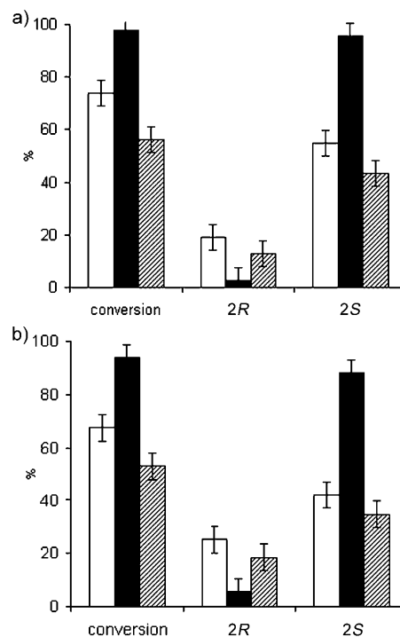
Figure 2. Conversion and product distribution of a) 4-methoxycyclohex-3-enecarbaldehyde ( 2a ) with 80 U mmol -1 after 5 min and b) 4-trimethylsilyloxycyclohex-3-enecarbaldehyde ( 2b ) with 150 U mmol -1 after 6 h with HbHNL enzyme variants (white = wild type, black = W128A, shaded = W128F).
