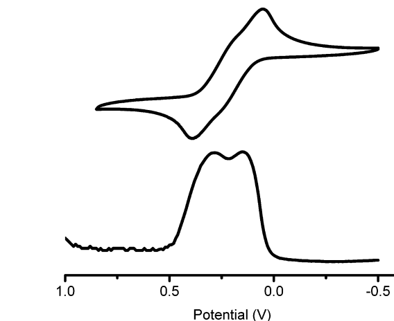
Figure 3. Cyclic and differential pulse voltammograms (CV and DPV) of 2 in a 0.1 M dichloromethane solution of (\text{Bu}_4\text{N})(\text{PF}_6) . The scan rate is 100 \text{ mV s}^{-1} for CV and 20 \text{ mV s}^{-1} for DPV.
