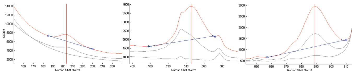
Figure 5. Raman bands: \text{POCl}_3 deformation ( 204\text{ cm}^{-1} ), P-Cl stretch ( 546\text{ cm}^{-1} ), P-O stretch ( 889\text{ cm}^{-1} ).
