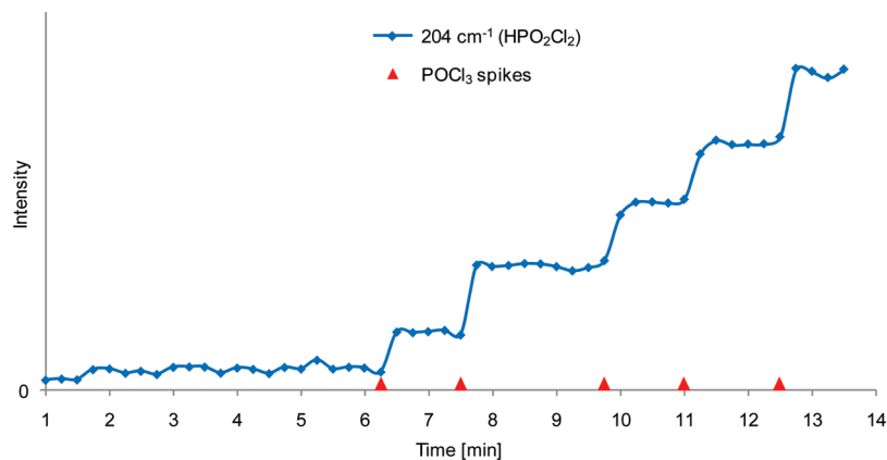
Figure 8. Limit of detection of phosphorodichloridic acid by in situ Raman ( \leq 0.015\text{ M} at 204\text{ cm}^{-1} ).
