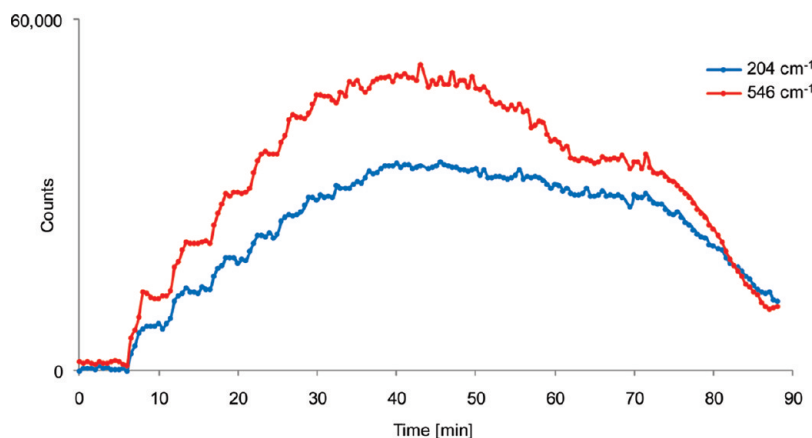
Figure 6. Phosphorodichloridic acid (2) monitored by Raman at 204\text{ cm}^{-1} and 546\text{ cm}^{-1} .
