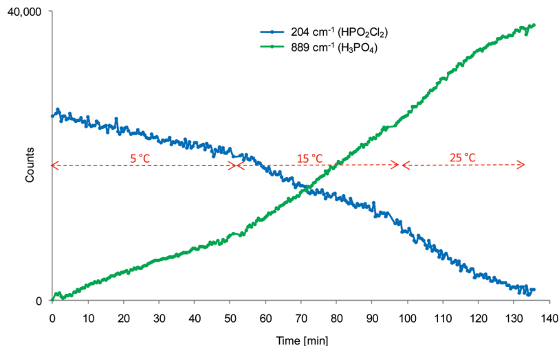
Figure 7. Effect of temperature on hydrolysis of \text{HPO}_2\text{Cl}_2 monitored by Raman.
