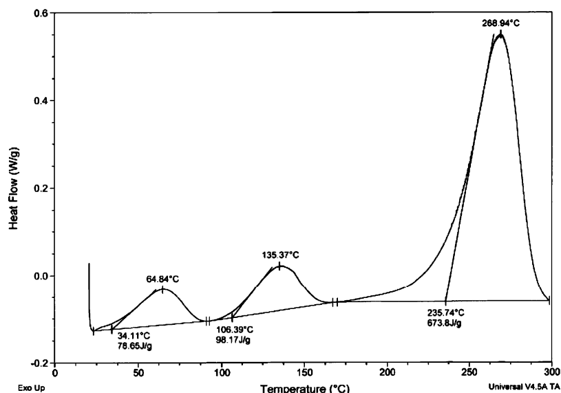
Figure 10. DSC after \text{POCl}_3 addition to mixture of acetonitrile/water at 0\text{--}5\text{ }^\circ\text{C} .
