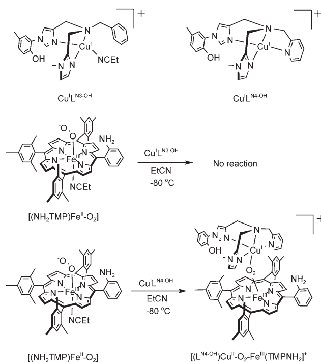
Scheme 4. Reaction behavior of the untethered heme superoxide [(\text{NH}_2\text{TMP})\text{Fe}^{\text{II}}\text{-(O}_2^-)] with the copper(I) components [\text{Cu}^{\text{I}}\text{L}^{\text{N3-OH}}]^+ and [\text{Cu}^{\text{I}}\text{L}^{\text{N4-OH}}]^+ .
