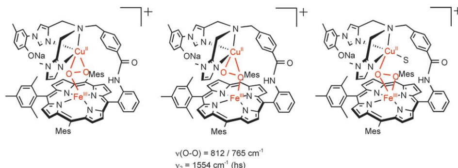
Figure 10. Possible dioxygen binding modes for the peroxide [(\text{L}^{\text{N3-ONa}})\text{Cu}^{\text{II}}\text{-O}_2\text{-Fe}^{\text{III}}(\text{TMP})]^+ .
