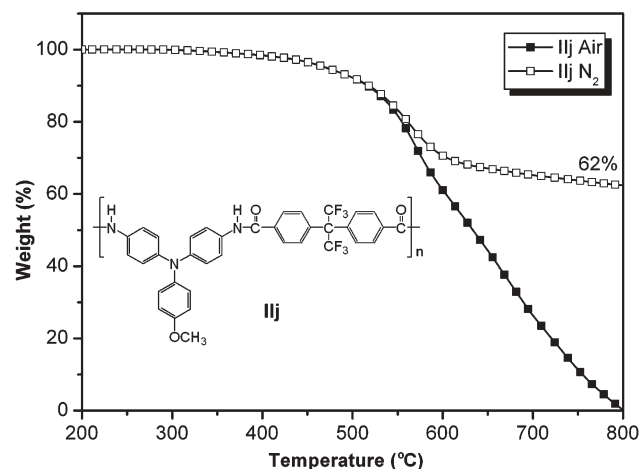
Fig. 5 TGA thermograms of polyamide II'j at a scan rate of 20\text{ }^{\circ}\text{C min}^{-1} .
