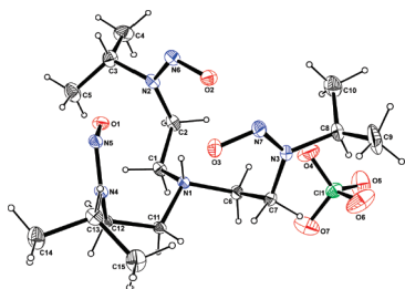
Figure 3. ORTEP diagram of L 1 ' perchlorate.
