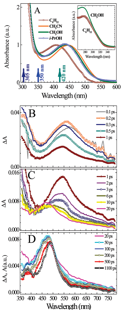
Figure 1. (A) UV-vis absorption spectra of azide 5 in several solvents ( \epsilon(445) = 1390 \text{ M}^{-1} \text{ cm}^{-1} in \text{CH}_3\text{CN} ) normalized to unity at the visible absorption maximum. The UV part of the spectrum is shown in the inset. The arrows indicate the excitation wavelengths used in the current study. (B–D) Transient absorption ( \Delta A ) spectra of a 16 mM solution of azide 5 in i -PrOH shown for various delay times between the 350 nm pump and probe pulses. The solution was flowed through a 0.5 mm flow cell and excited with 4 \mu\text{J} pulses. The delay times in picoseconds are shown in the frame legends: B (short times, 0.1–1 ps), C (intermediate times, 1–20 ps), and D (long times, 20–1100 ps). Data in D represent smoothed spectra by adjacent-averaging (bandwidth, 3.5 nm). The solvent contribution to the \Delta A spectra is minor at delay times equal to or longer than 100 fs, except for the 388.9 nm feature that corresponds to stimulated Raman scattering from i -PrOH and yields 11 the instrument response function, 150 fs (fwhm).
