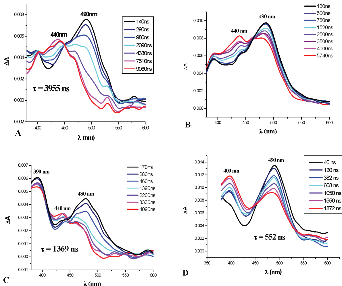
Figure 11. Spectroscopic properties in the nanosecond–microsecond time domain of azide 5 in (A) dimethyl malonate, (B) dimethylamine hydrochloride, (C) phenol, and (D) hydroquinone with the last three spectra acquired in acetonitrile.
