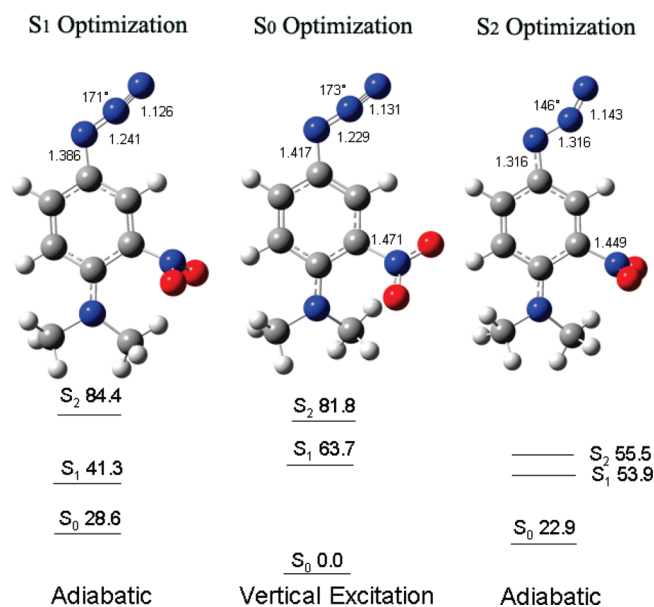
Figure 7. Excited state energies (kcal/mol) and bond lengths for the optimized geometries (TD-B3LYP) of the ground state, and the first and second excited states of the N,N -dimethyl analogue of azide 5 .
