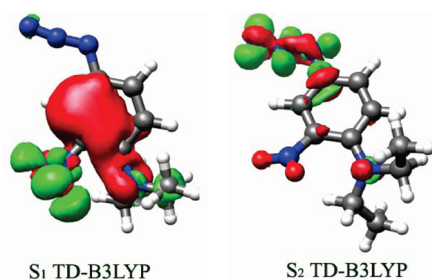
Figure 6. Electron density redistribution in the (left) S 1 and (right) S 2 states of 5 calculated at the TD-B3LYP/TZVP level of theory. The green contours depict the accumulation of electron density in the excited state, and the red contours illustrate the loss of electron density from the S 0 ground state. The contour values are \pm 0.005 au.
