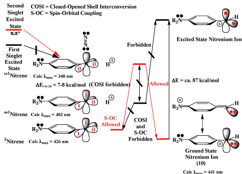
Figure 9. Possible reaction pathways connecting excited states of azide 5 , nitrene states, and nitrenium ion ( 10 ) states. The vertical energy axis is not drawn to scale.
