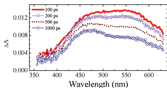
Figure 5. Long-time transient absorption ( \Delta A ) spectra of azide 5 in toluene upon 350 nm excitation. The solution (16 mM) was circulated through a 0.5 mm path length flow cell.
