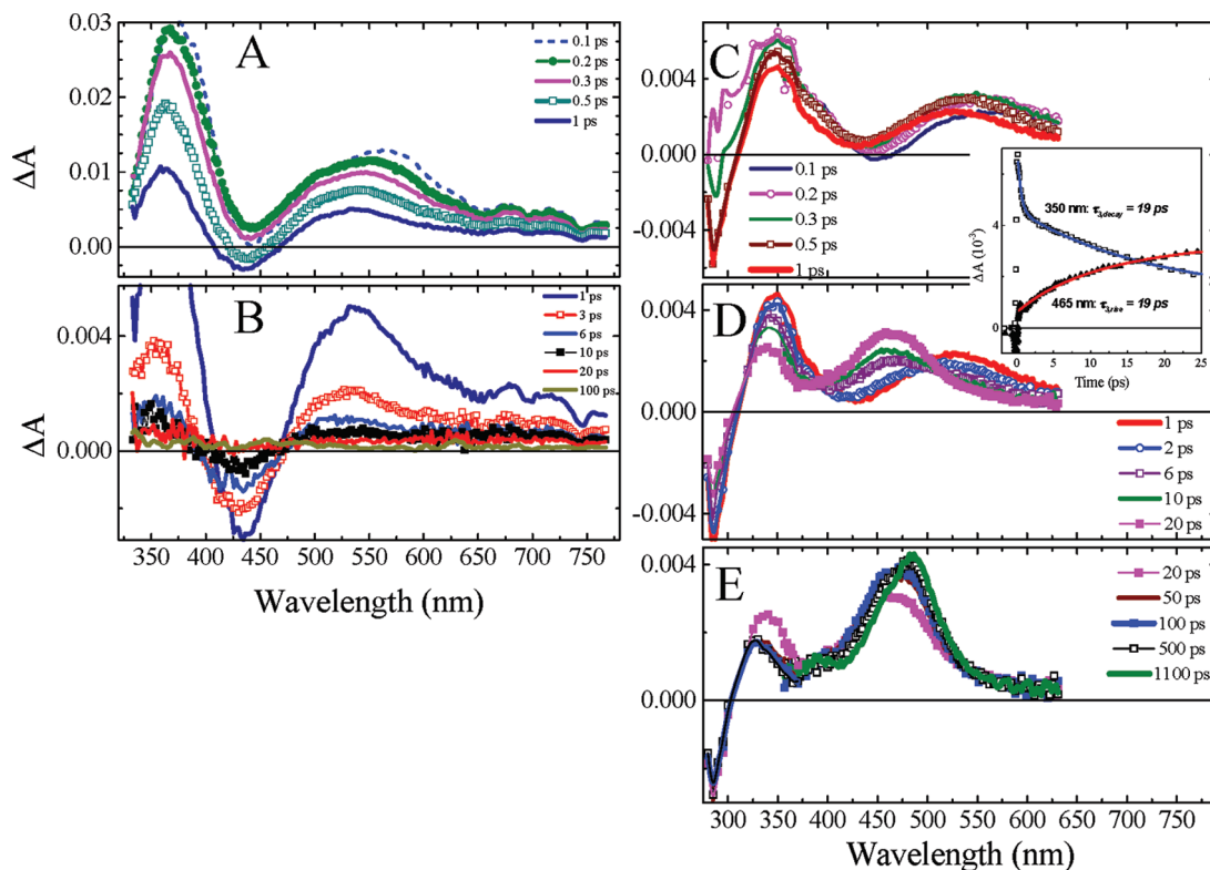
Figure 3. Transient absorption ( \Delta A ) spectra of azide 5 (1.2 mM) in i -PrOH for various delay times (in picoseconds, shown in the legends) between the probe and pump pulses. (A,B) Solution was flowed through a 0.5 mm flow cell and excited with a 420 nm, 3.5 \mu J pulse. (C–E) Solution was flowed through a 0.2 mm flow cell and excited with a 305 nm, 3.8 \mu J pulse. The solvent contribution to the \Delta A spectra is minor at delay times \geq 100 fs; see Figure SM1 in Supporting Information. For 305 nm excitation, the UV region (280–375 nm) of the \Delta A spectra was measured using the probe light generated by TOPAS ([azide 5 ] = 1.7 mM, 3.1 \mu J pump pulse) and subsequently scaled to the visible (360–665 nm) \Delta A spectra measured using the white-light continuum probe. The inset compares the \Delta A kinetic traces recorded at probe wavelengths of 350 and 465 nm.
