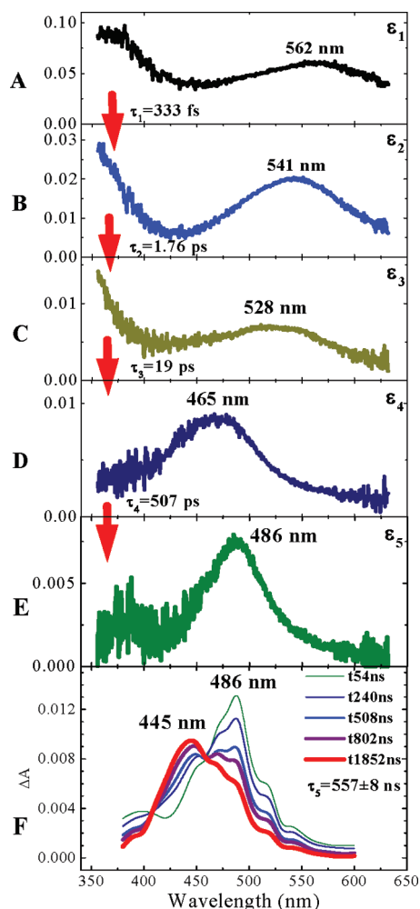
Figure 4. Reconstructed decay-associated spectra ( \epsilon_i ) extracted from the \Delta A transient absorption spectra of azide 5 in i -PrOH irradiated with 350 nm laser pulses. The time constants ( \tau_i ) obtained from a least-squares global fit of the 512 \Delta A kinetic traces to a sum of four exponential functions and a permanent offset are shown in the insets. (A) Absorption of excited electronic state of azide 5 ; (B) hot ground state of 5 following internal conversion; (C) hot singlet nitrene and probably residual hot ground state of azide 5 at 528 nm; (D) triplet nitrene and nitrenium ion 10 ; (E) nitrenium ion 10 ; (F) ns/ \mu s decay of the nitrenium ion 10 (486 nm) and formation of the adduct 14 (445 nm).
