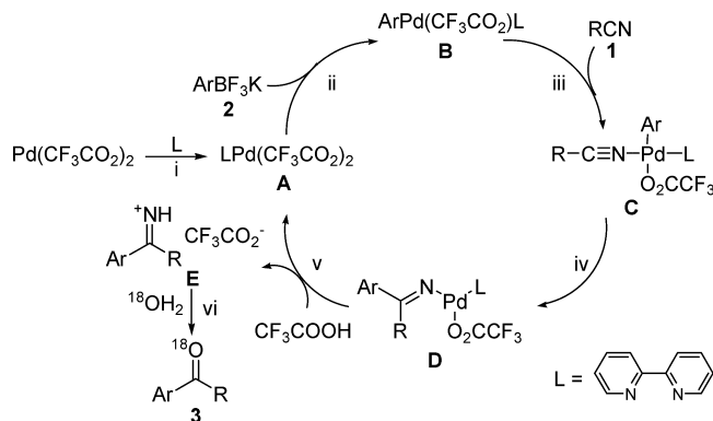
Scheme 3. Plausible Mechanism
