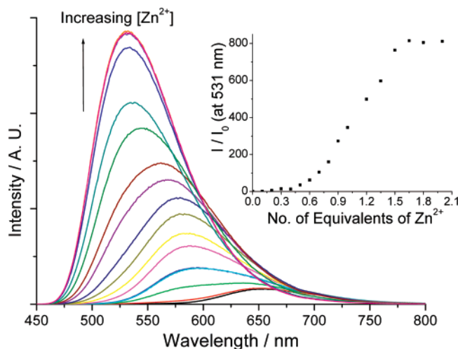
Figure 9. Emission spectral traces and (inset) emission intensity enhancement factor ( I/I_0 , monitored at 531 nm) of 2e at increasing equivalents of \text{Zn}(\text{NO}_3)_2 in 0.1 M {}^n\text{Bu}_4\text{NPF}_6 methanolic solution at 298 K ( \lambda_{\text{ex}} = 420 nm, [\text{2e}] = 4.96 \times 10^{-5} M).
