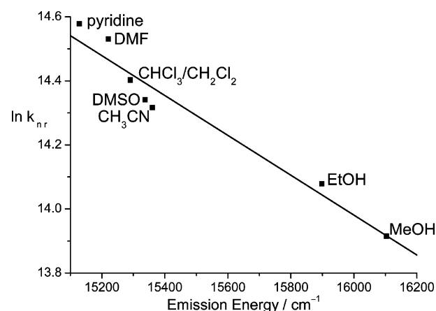
Figure 8. Plot of \ln k_{\text{nr}} against E_{\text{em}} for 2c in various solvents at 298 K.
